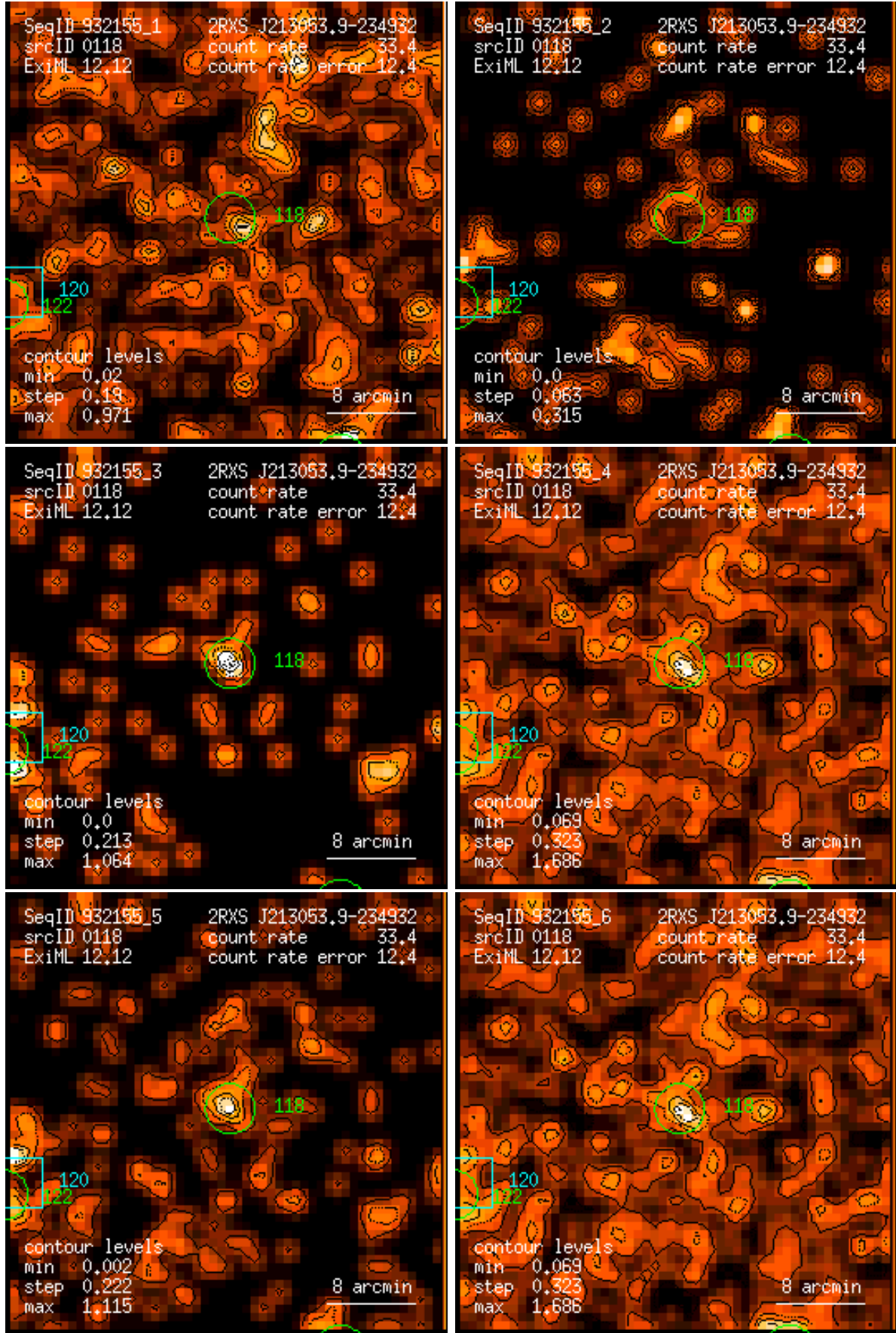
Figure 118: RASS 932155: detection 0118: band rate images, Gaussian filter: (1) PSPC channels 11 – 41, (2) 52 – 90, (3) 91 – 201, (4) 11 – 235, (5) 52 – 201, (6) 11 – 201. Broad band rates in counts/ks. Band rate contour levels in counts/ks/arcmin 2 .
