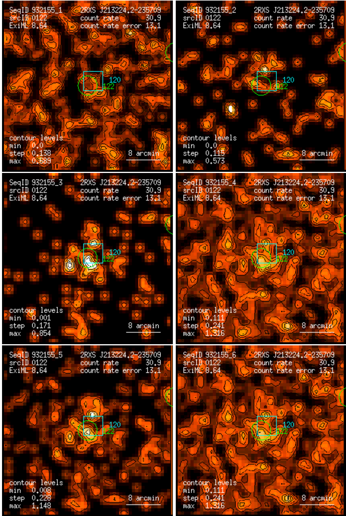
Figure 122: RASS 932155: detection 0122: band rate images, Gaussian filter: (1) PSPC channels 11 – 41, (2) 52 – 90, (3) 91 – 201, (4) 11 – 235, (5) 52 – 201, (6) 11 – 201. Broad band rates in counts/ks. Band rate contour levels in counts/ks/arcmin 2 .
