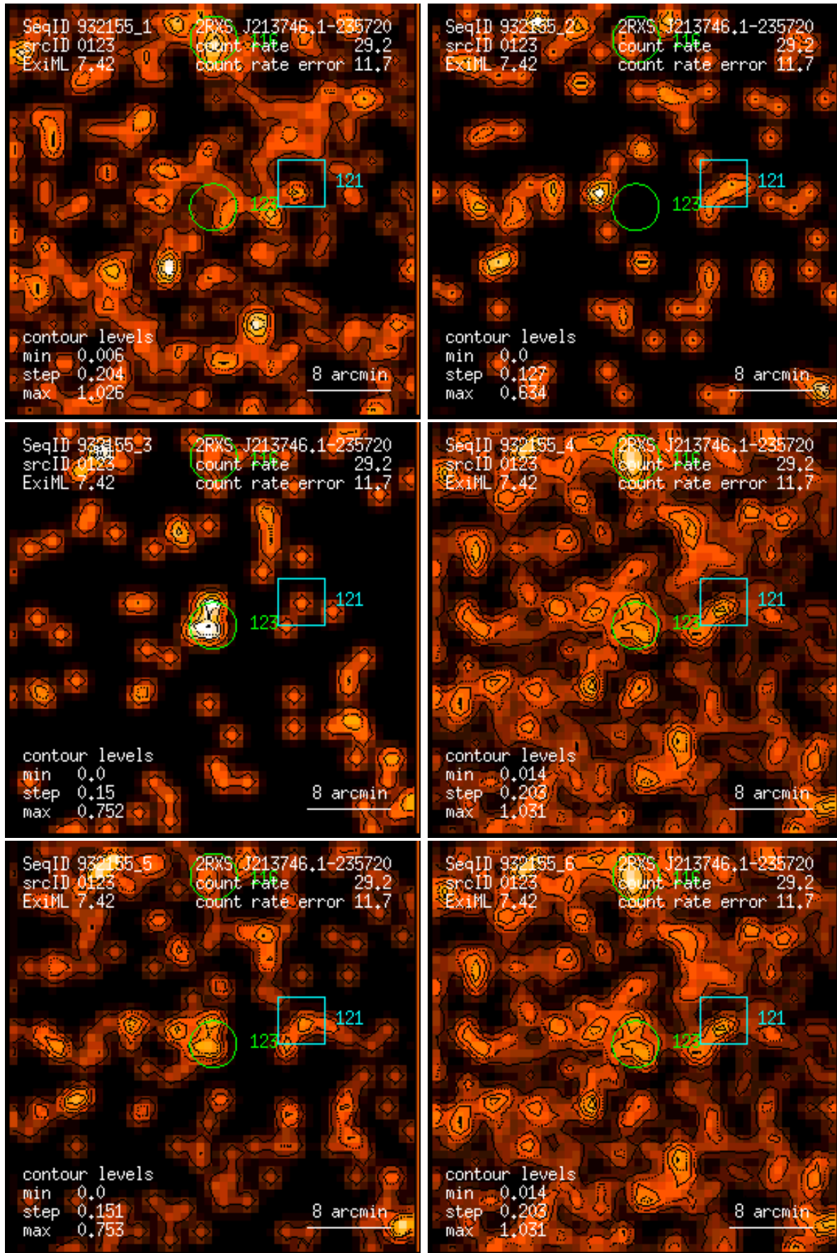
Figure 123: RASS 932155: detection 0123: band rate images, Gaussian filter: (1) PSPC channels 11 – 41, (2) 52 – 90, (3) 91 – 201, (4) 11 – 235, (5) 52 – 201, (6) 11 – 201. Broad band rates in counts/ks. Band rate contour levels in counts/ks/arcmin 2 .
