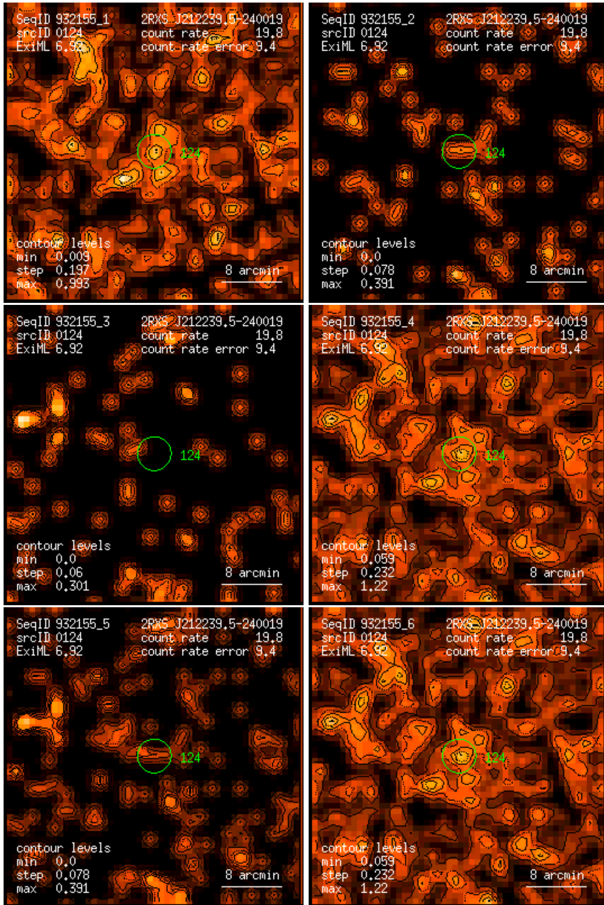
Figure 124: RASS 932155: detection 0124: band rate images, Gaussian filter: (1) PSPC channels 11 – 41, (2) 52 – 90, (3) 91 – 201, (4) 11 – 235, (5) 52 – 201, (6) 11 – 201. Broad band rates in counts/ks. Band rate contour levels in counts/ks/arcmin 2 .
