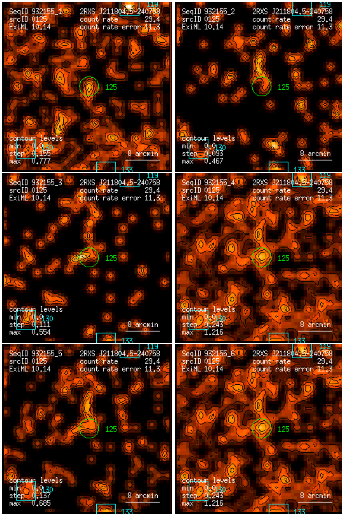
Figure 125: RASS 932155: detection 0125: band rate images, Gaussian filter: (1) PSPC channels 11 – 41, (2) 52 – 90, (3) 91 – 201, (4) 11 – 235, (5) 52 – 201, (6) 11 – 201. Broad band rates in counts/ks. Band rate contour levels in counts/ks/arcmin 2 .
