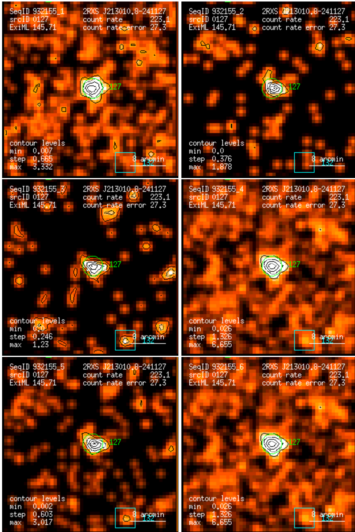
Figure 127: RASS 932155: detection 0127: band rate images, Gaussian filter: (1) PSPC channels 11 – 41, (2) 52 – 90, (3) 91 – 201, (4) 11 – 235, (5) 52 – 201, (6) 11 – 201. Broad band rates in counts/ks. Band rate contour levels in counts/ks/arcmin 2 .
