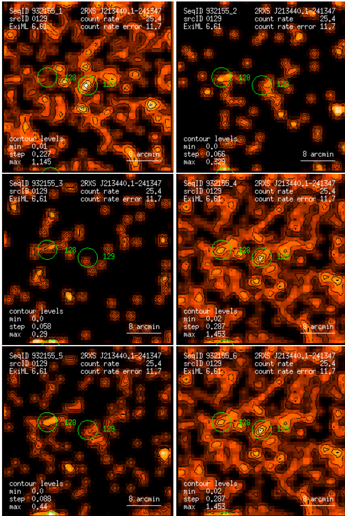
Figure 129: RASS 932155: detection 0129: band rate images, Gaussian filter: (1) PSPC channels 11 – 41, (2) 52 – 90, (3) 91 – 201, (4) 11 – 235, (5) 52 – 201, (6) 11 – 201. Broad band rates in counts/ks. Band rate contour levels in counts/ks/arcmin 2 .
