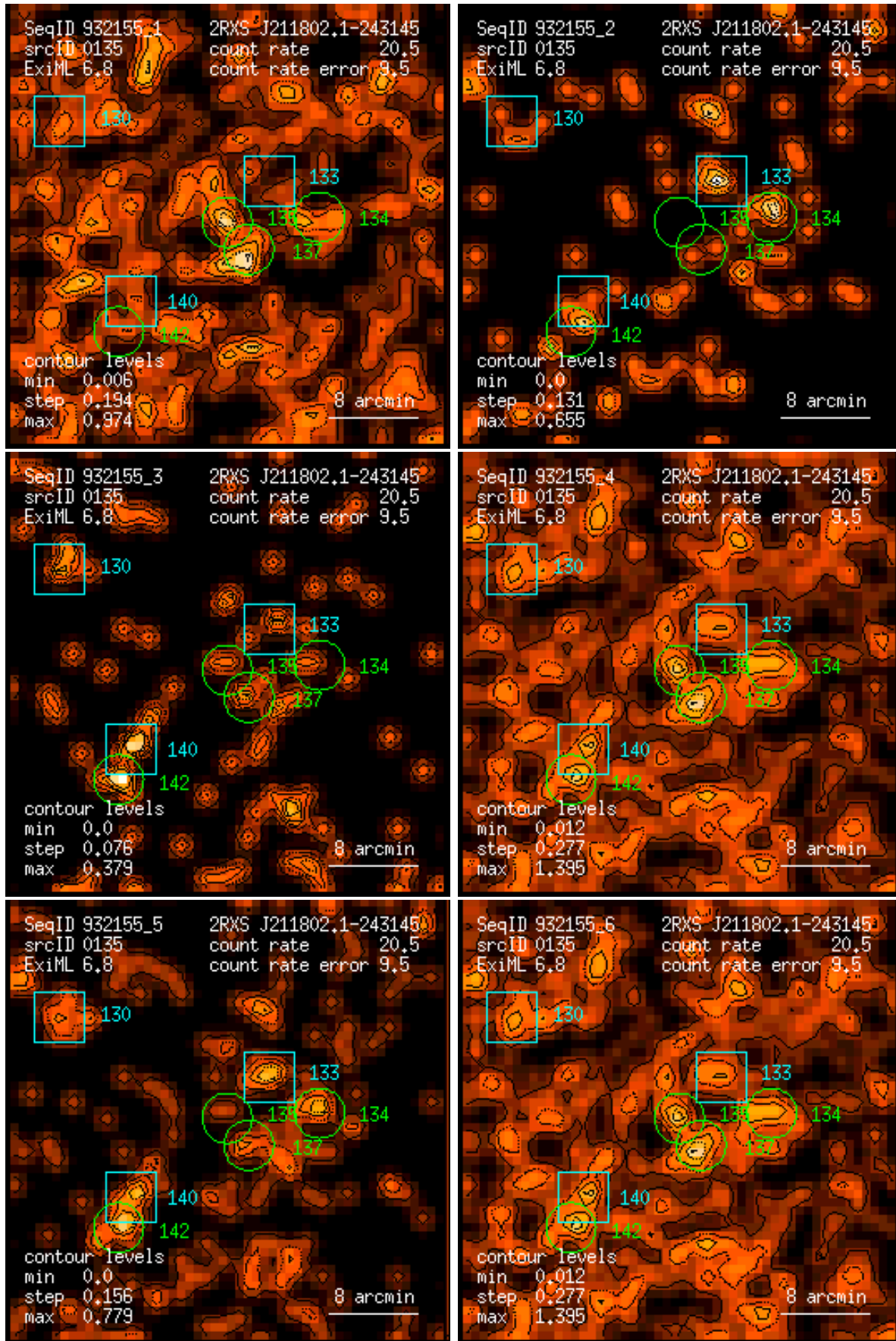
Figure 135: RASS 932155: detection 0135: band rate images, Gaussian filter: (1) PSPC channels 11 – 41, (2) 52 – 90, (3) 91 – 201, (4) 11 – 235, (5) 52 – 201, (6) 11 – 201. Broad band rates in counts/ks. Band rate contour levels in counts/ks/arcmin 2 .
