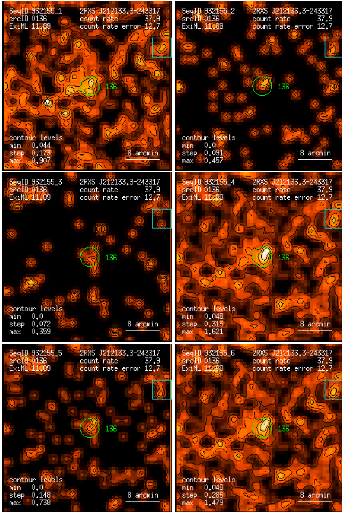
Figure 136: RASS 932155: detection 0136: band rate images, Gaussian filter: (1) PSPC channels 11 – 41, (2) 52 – 90, (3) 91 – 201, (4) 11 – 235, (5) 52 – 201, (6) 11 – 201. Broad band rates in counts/ks. Band rate contour levels in counts/ks/arcmin 2 .
