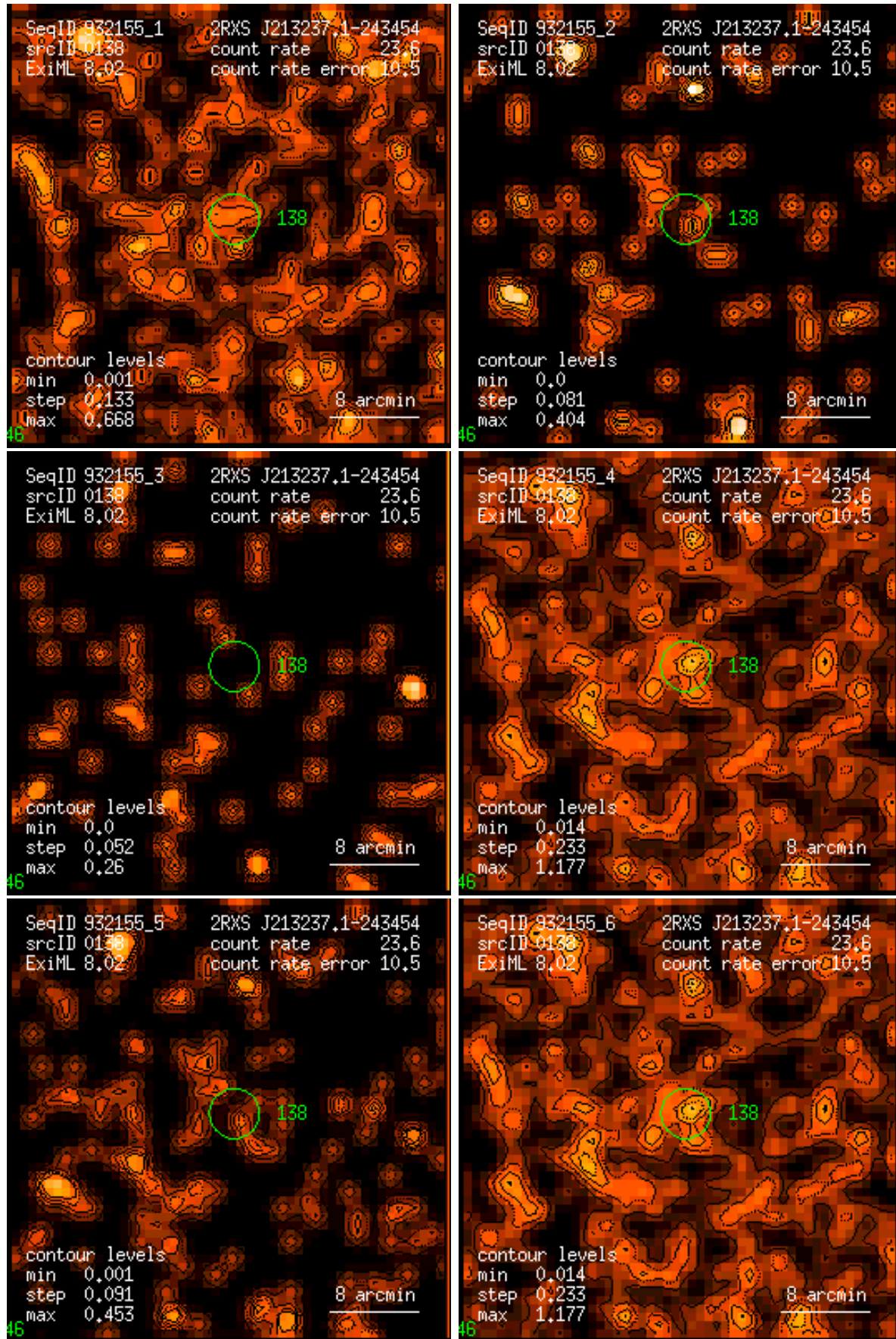
Figure 138: RASS 932155: detection 0138: band rate images, Gaussian filter: (1) PSPC channels 11 – 41, (2) 52 – 90, (3) 91 – 201, (4) 11 – 235, (5) 52 – 201, (6) 11 – 201. Broad band rates in counts/ks. Band rate contour levels in counts/ks/arcmin 2 .
