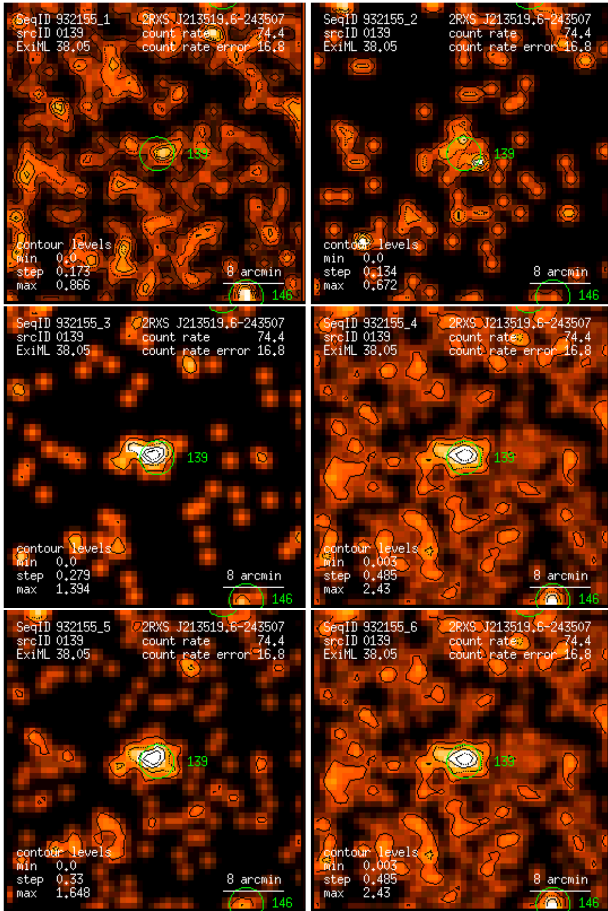
Figure 139: RASS 932155: detection 0139: band rate images, Gaussian filter: (1) PSPC channels 11 – 41, (2) 52 – 90, (3) 91 – 201, (4) 11 – 235, (5) 52 – 201, (6) 11 – 201. Broad band rates in counts/ks. Band rate contour levels in counts/ks/arcmin 2 .
