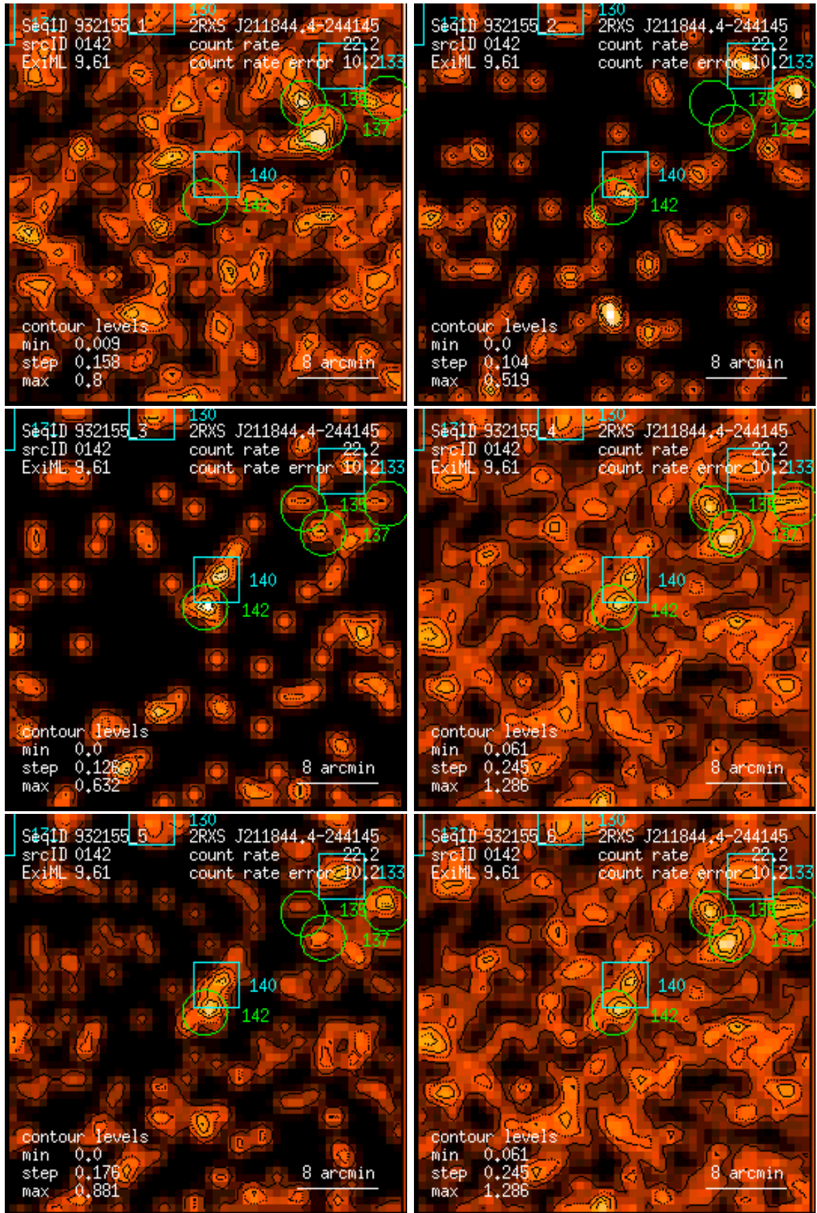
Figure 142: RASS 932155: detection 0142: band rate images, Gaussian filter: (1) PSPC channels 11 – 41, (2) 52 – 90, (3) 91 – 201, (4) 11 – 235, (5) 52 – 201, (6) 11 – 201. Broad band rates in counts/ks. Band rate contour levels in counts/ks/arcmin 2 .
