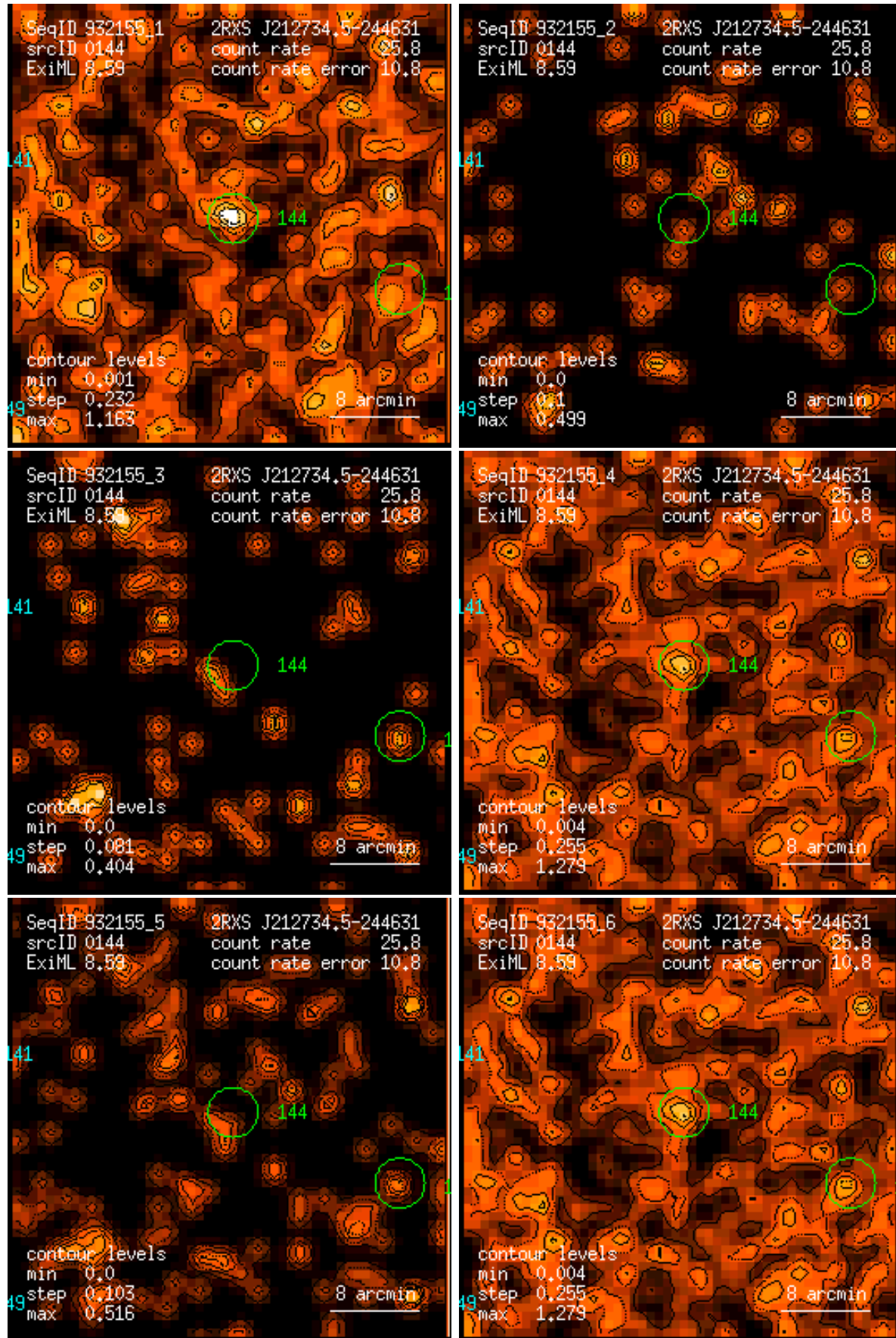
Figure 144: RASS 932155: detection 0144: band rate images, Gaussian filter: (1) PSPC channels 11 – 41, (2) 52 – 90, (3) 91 – 201, (4) 11 – 235, (5) 52 – 201, (6) 11 – 201. Broad band rates in counts/ks. Band rate contour levels in counts/ks/arcmin 2 .
