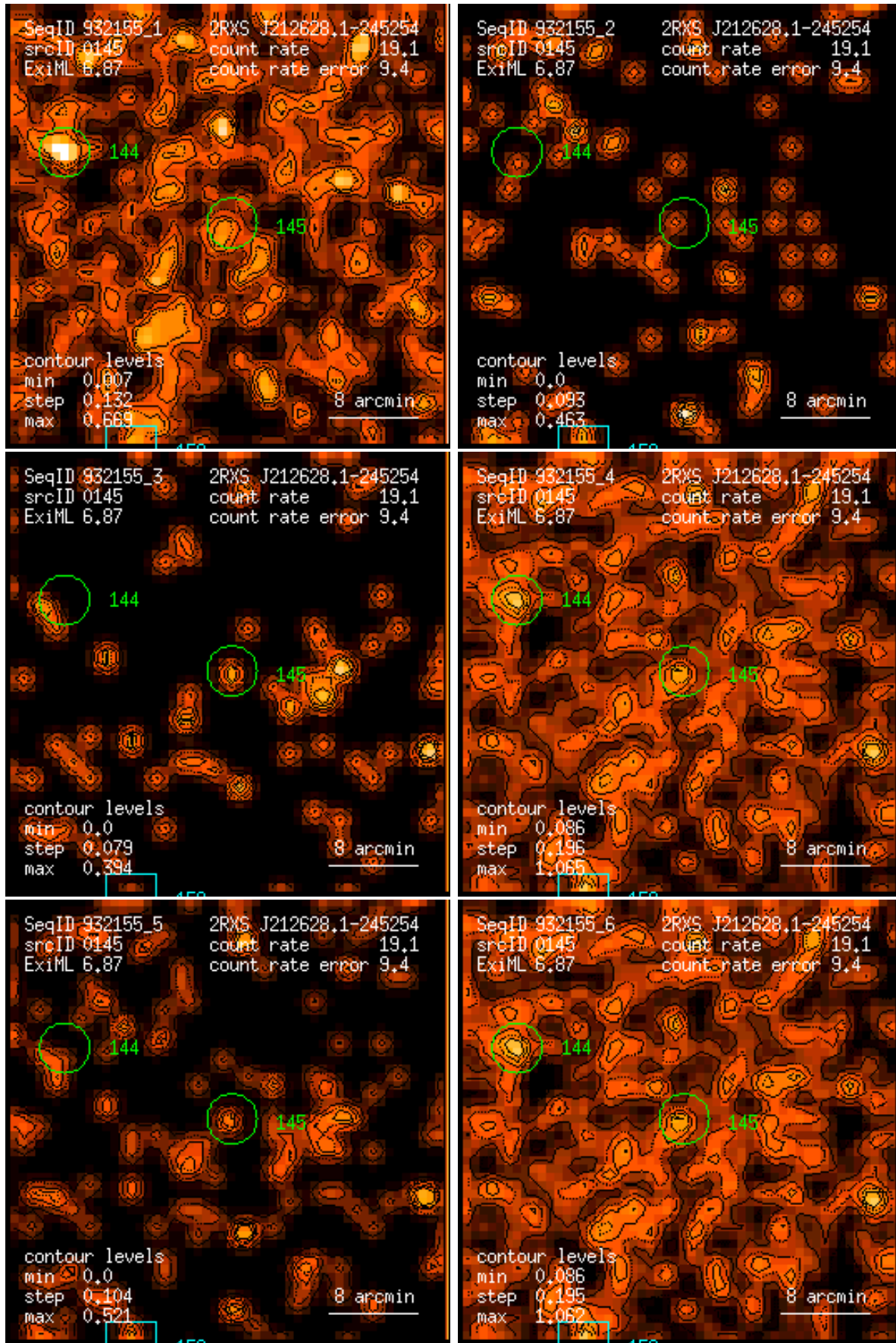
Figure 145: RASS 932155: detection 0145: band rate images, Gaussian filter: (1) PSPC channels 11 – 41, (2) 52 – 90, (3) 91 – 201, (4) 11 – 235, (5) 52 – 201, (6) 11 – 201. Broad band rates in counts/ks. Band rate contour levels in counts/ks/arcmin 2 .
