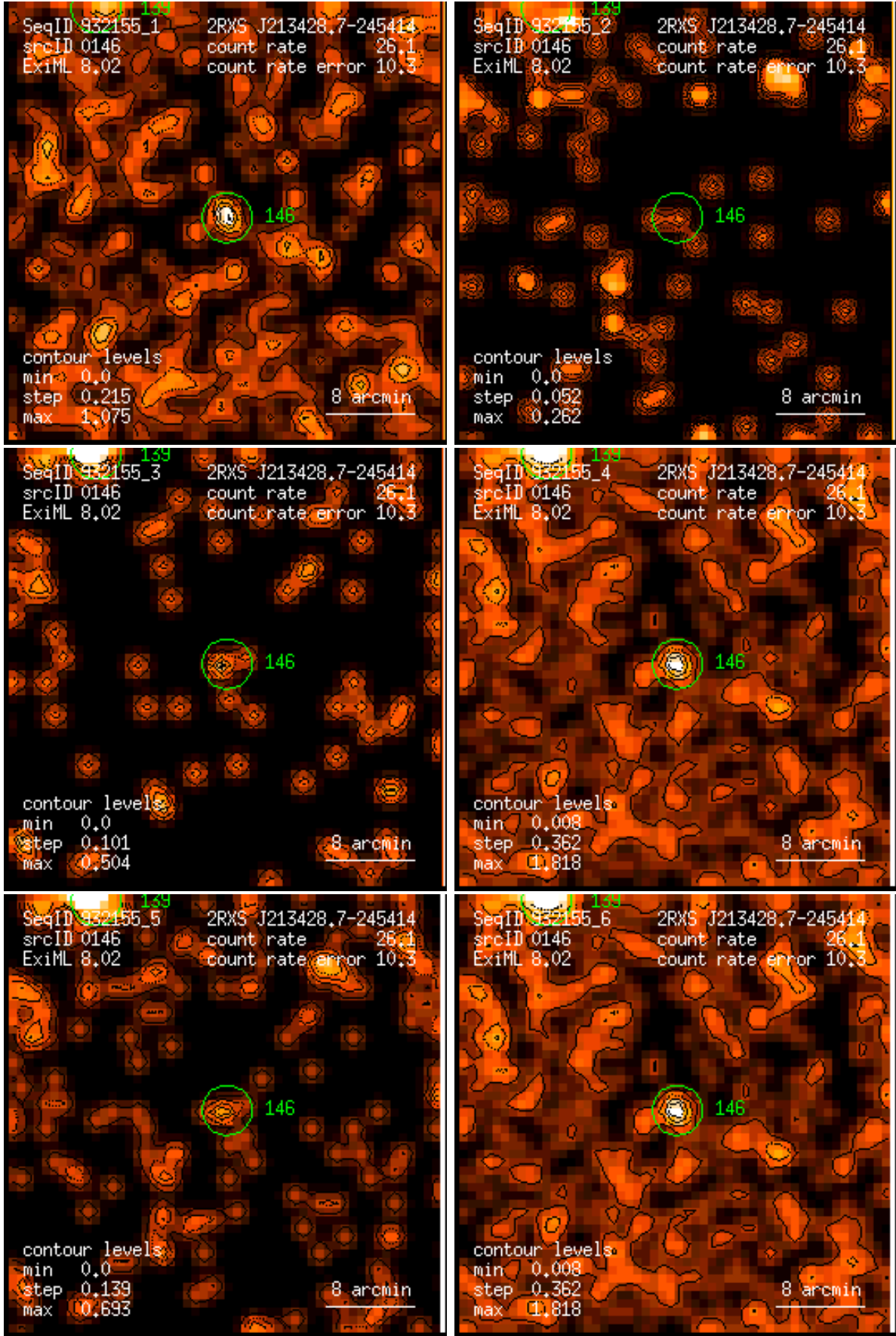
Figure 146: RASS 932155: detection 0146: band rate images, Gaussian filter: (1) PSPC channels 11 – 41, (2) 52 – 90, (3) 91 – 201, (4) 11 – 235, (5) 52 – 201, (6) 11 – 201. Broad band rates in counts/ks. Band rate contour levels in counts/ks/arcmin 2 .
