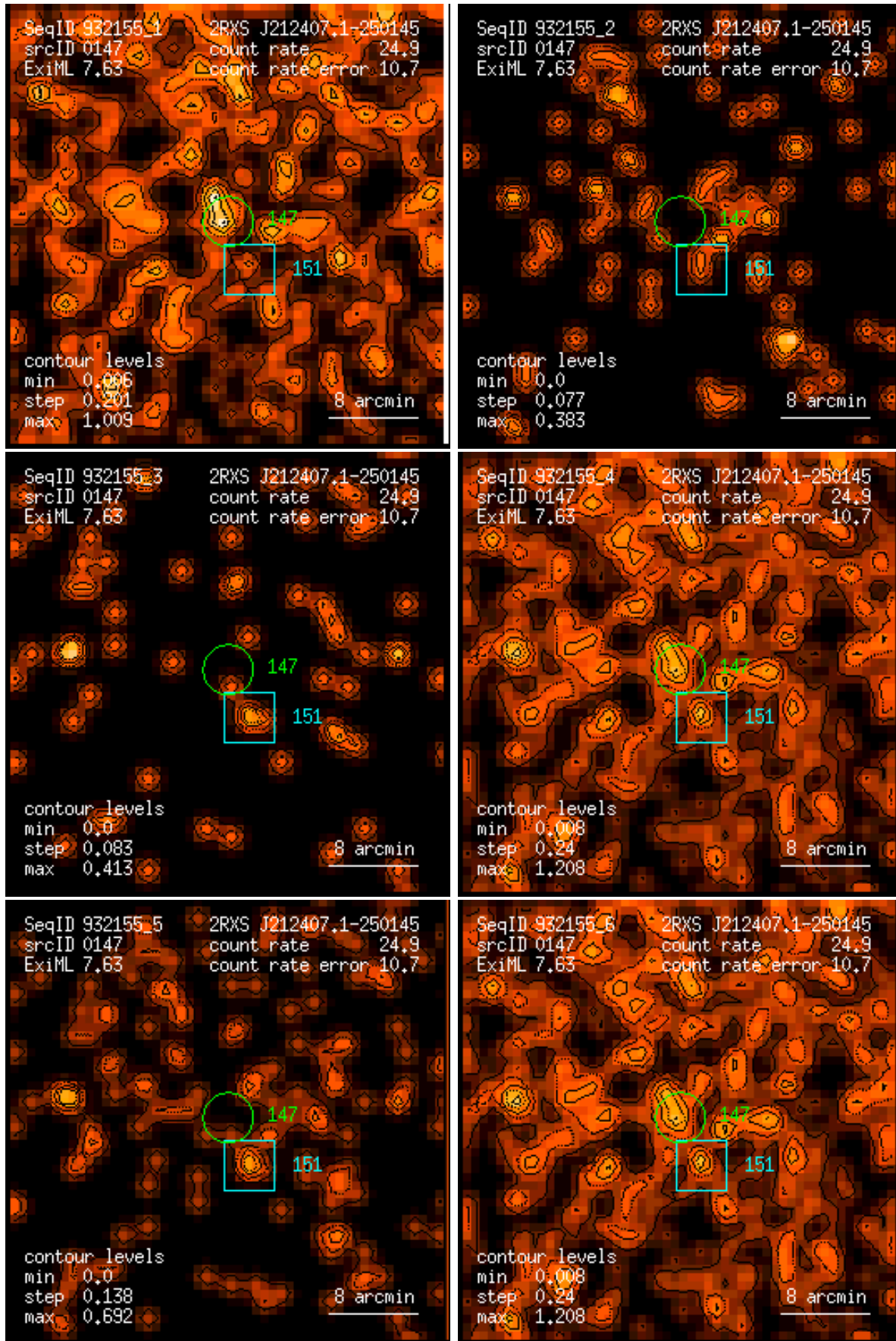
Figure 147: RASS 932155: detection 0147: band rate images, Gaussian filter: (1) PSPC channels 11 – 41, (2) 52 – 90, (3) 91 – 201, (4) 11 – 235, (5) 52 – 201, (6) 11 – 201. Broad band rates in counts/ks. Band rate contour levels in counts/ks/arcmin 2 .
