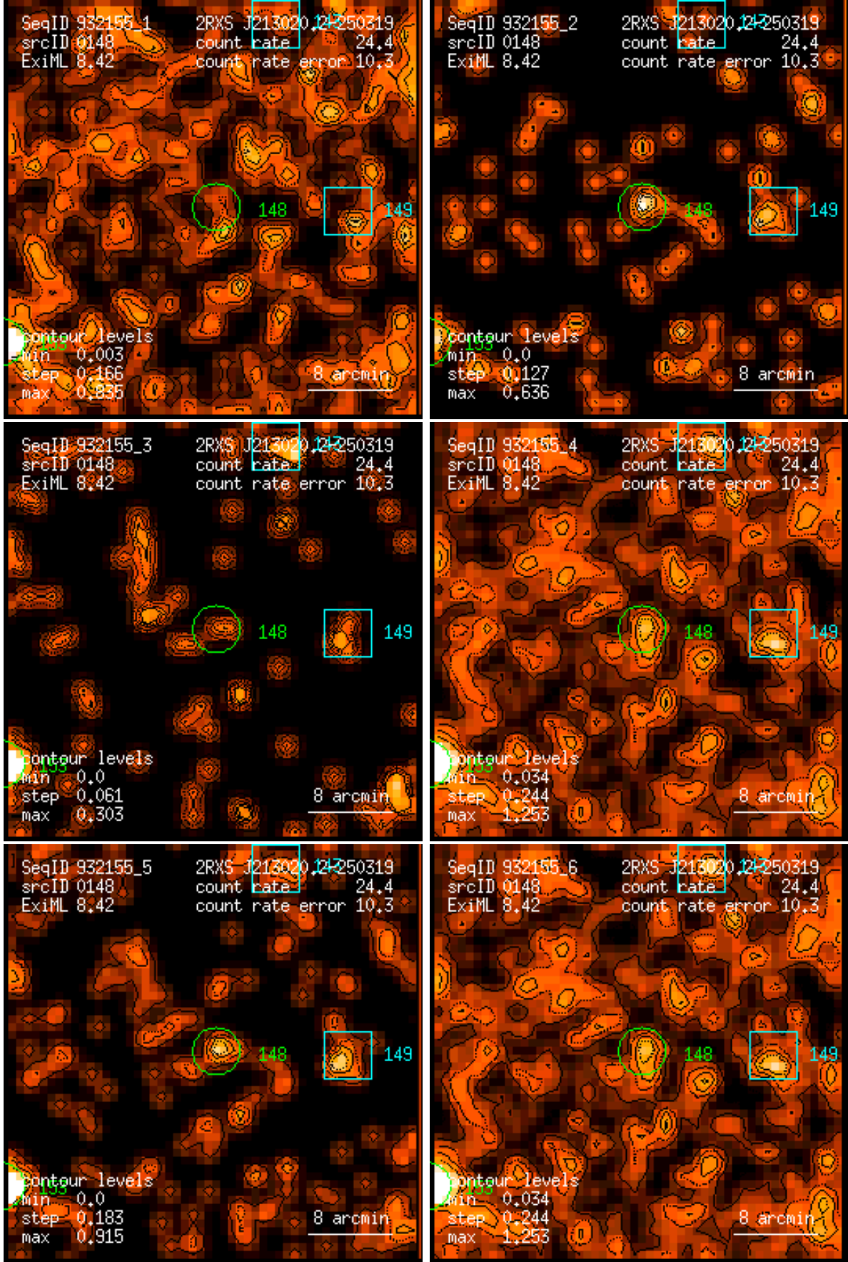
Figure 148: RASS 932155: detection 0148: band rate images, Gaussian filter: (1) PSPC channels 11 – 41, (2) 52 – 90, (3) 91 – 201, (4) 11 – 235, (5) 52 – 201, (6) 11 – 201. Broad band rates in counts/ks. Band rate contour levels in counts/ks/arcmin 2 .
