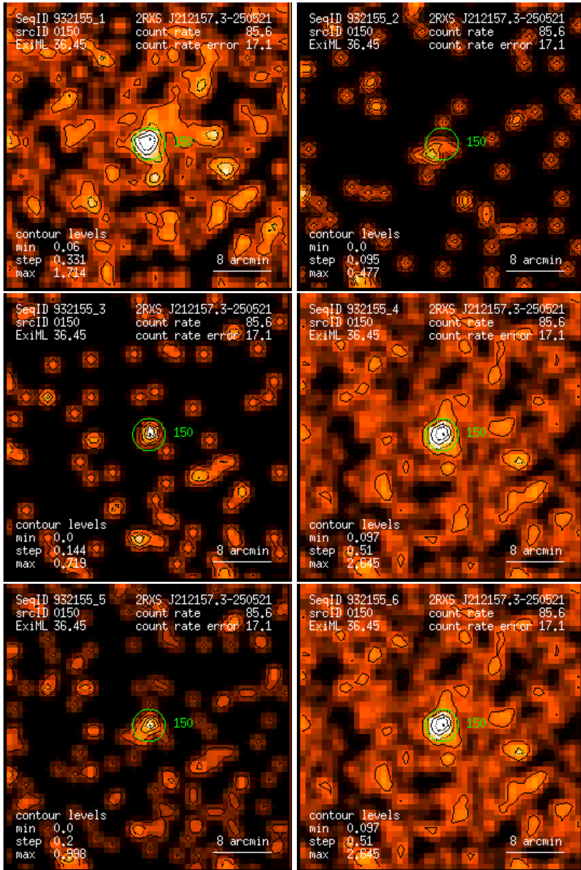
Figure 150: RASS 932155: detection 0150: band rate images, Gaussian filter: (1) PSPC channels 11 – 41, (2) 52 – 90, (3) 91 – 201, (4) 11 – 235, (5) 52 – 201, (6) 11 – 201. Broad band rates in counts/ks. Band rate contour levels in counts/ks/arcmin 2 .
