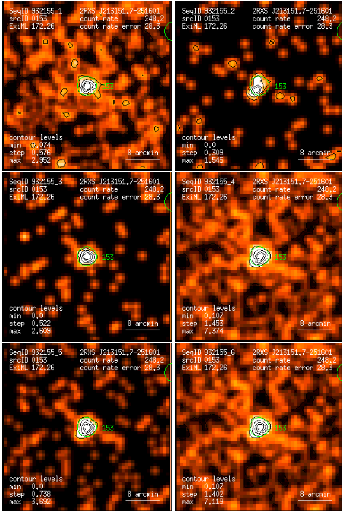
Figure 153: RASS 932155: detection 0153: band rate images, Gaussian filter: (1) PSPC channels 11 – 41, (2) 52 – 90, (3) 91 – 201, (4) 11 – 235, (5) 52 – 201, (6) 11 – 201. Broad band rates in counts/ks. Band rate contour levels in counts/ks/arcmin 2 .
