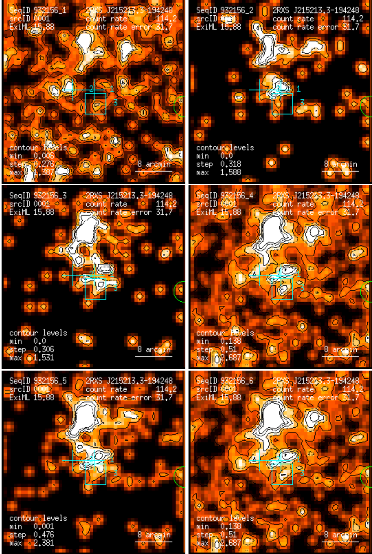
Figure 1: RASS 932156: detection 0001: band rate images, Gaussian filter: (1) PSPC channels 11 – 41, (2) 52 – 90, (3) 91 – 201, (4) 11 – 235, (5) 52 – 201, (6) 11 – 201. Broad band rates in counts/ks. Band rate contour levels in counts/ks/arcmin 2 .
