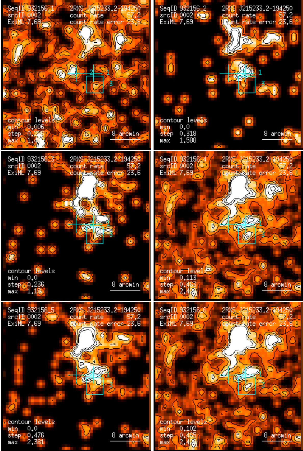
Figure 2: RASS 932156: detection 0002: band rate images, Gaussian filter: (1) PSPC channels 11 – 41, (2) 52 – 90, (3) 91 – 201, (4) 11 – 235, (5) 52 – 201, (6) 11 – 201. Broad band rates in counts/ks. Band rate contour levels in counts/ks/arcmin 2 .
