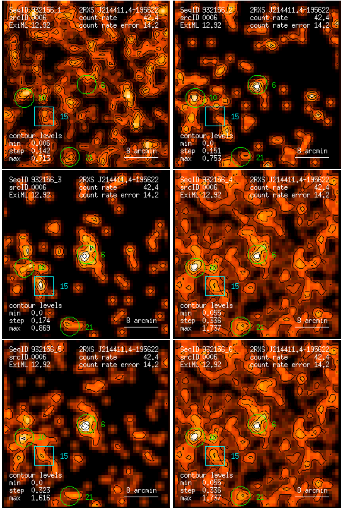
Figure 6: RASS 932156: detection 0006: band rate images, Gaussian filter: (1) PSPC channels 11 – 41, (2) 52 – 90, (3) 91 – 201, (4) 11 – 235, (5) 52 – 201, (6) 11 – 201. Broad band rates in counts/ks. Band rate contour levels in counts/ks/arcmin 2 .
