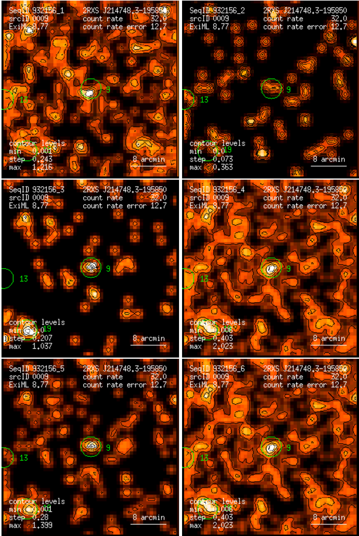
Figure 9: RASS 932156: detection 0009: band rate images, Gaussian filter: (1) PSPC channels 11 – 41, (2) 52 – 90, (3) 91 – 201, (4) 11 – 235, (5) 52 – 201, (6) 11 – 201. Broad band rates in counts/ks. Band rate contour levels in counts/ks/arcmin 2 .
