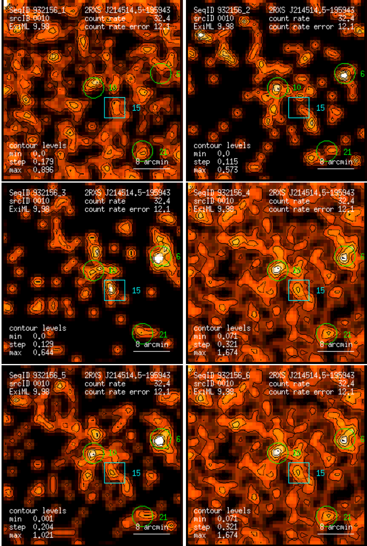
Figure 10: RASS 932156: detection 0010: band rate images, Gaussian filter: (1) PSPC channels 11 – 41, (2) 52 – 90, (3) 91 – 201, (4) 11 – 235, (5) 52 – 201, (6) 11 – 201. Broad band rates in counts/ks. Band rate contour levels in counts/ks/arcmin 2 .
