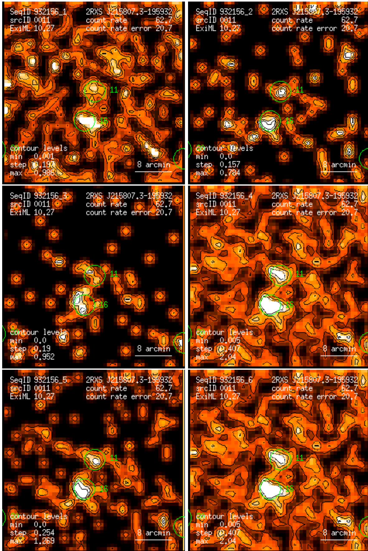
Figure 11: RASS 932156: detection 0011: band rate images, Gaussian filter: (1) PSPC channels 11 – 41, (2) 52 – 90, (3) 91 – 201, (4) 11 – 235, (5) 52 – 201, (6) 11 – 201. Broad band rates in counts/ks. Band rate contour levels in counts/ks/arcmin 2 .
