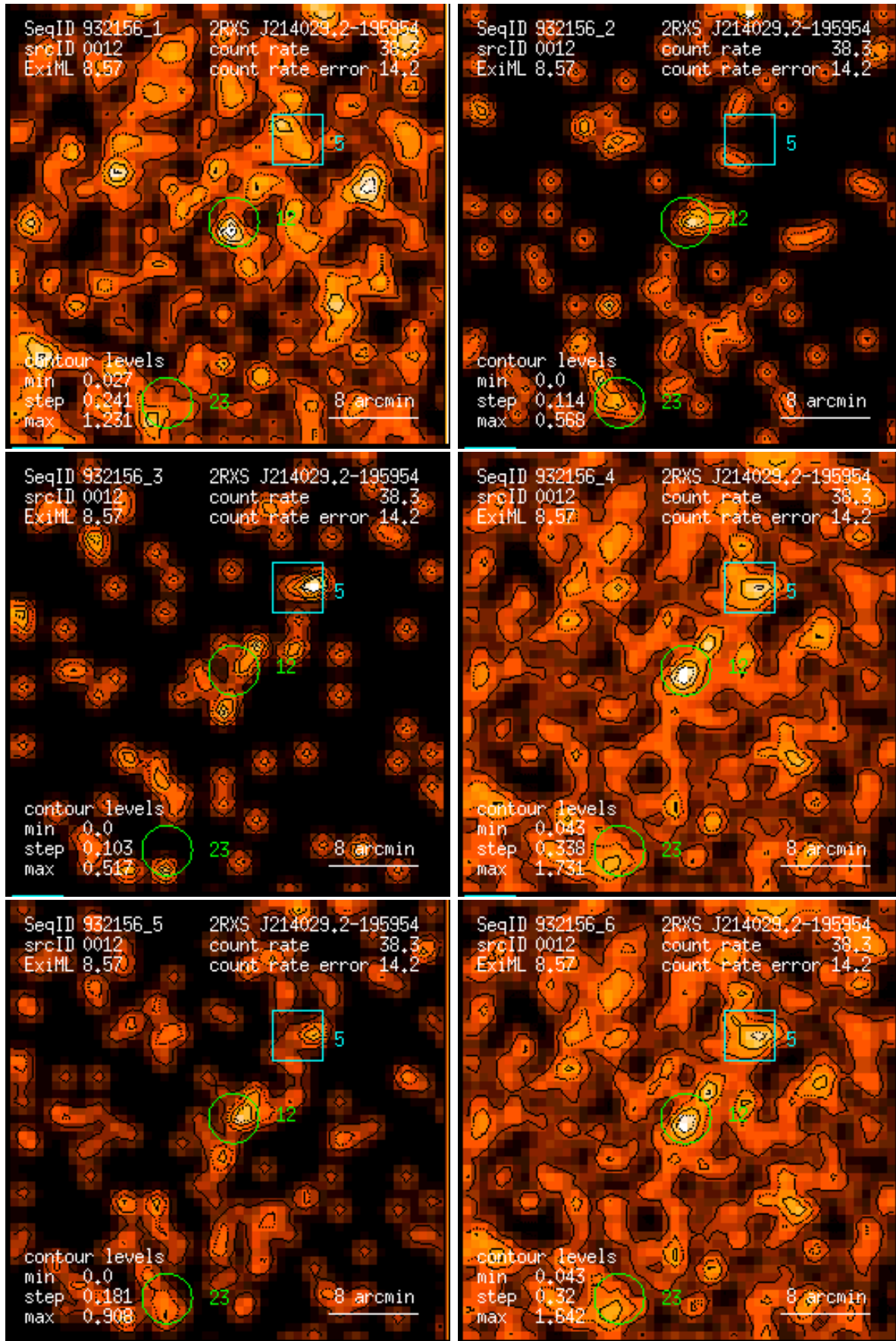
Figure 12: RASS 932156: detection 0012: band rate images, Gaussian filter: (1) PSPC channels 11 – 41, (2) 52 – 90, (3) 91 – 201, (4) 11 – 235, (5) 52 – 201, (6) 11 – 201. Broad band rates in counts/ks. Band rate contour levels in counts/ks/arcmin 2 .
