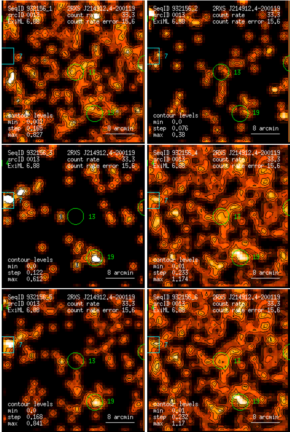
Figure 13: RASS 932156: detection 0013: band rate images, Gaussian filter: (1) PSPC channels 11 – 41, (2) 52 – 90, (3) 91 – 201, (4) 11 – 235, (5) 52 – 201, (6) 11 – 201. Broad band rates in counts/ks. Band rate contour levels in counts/ks/arcmin 2 .
