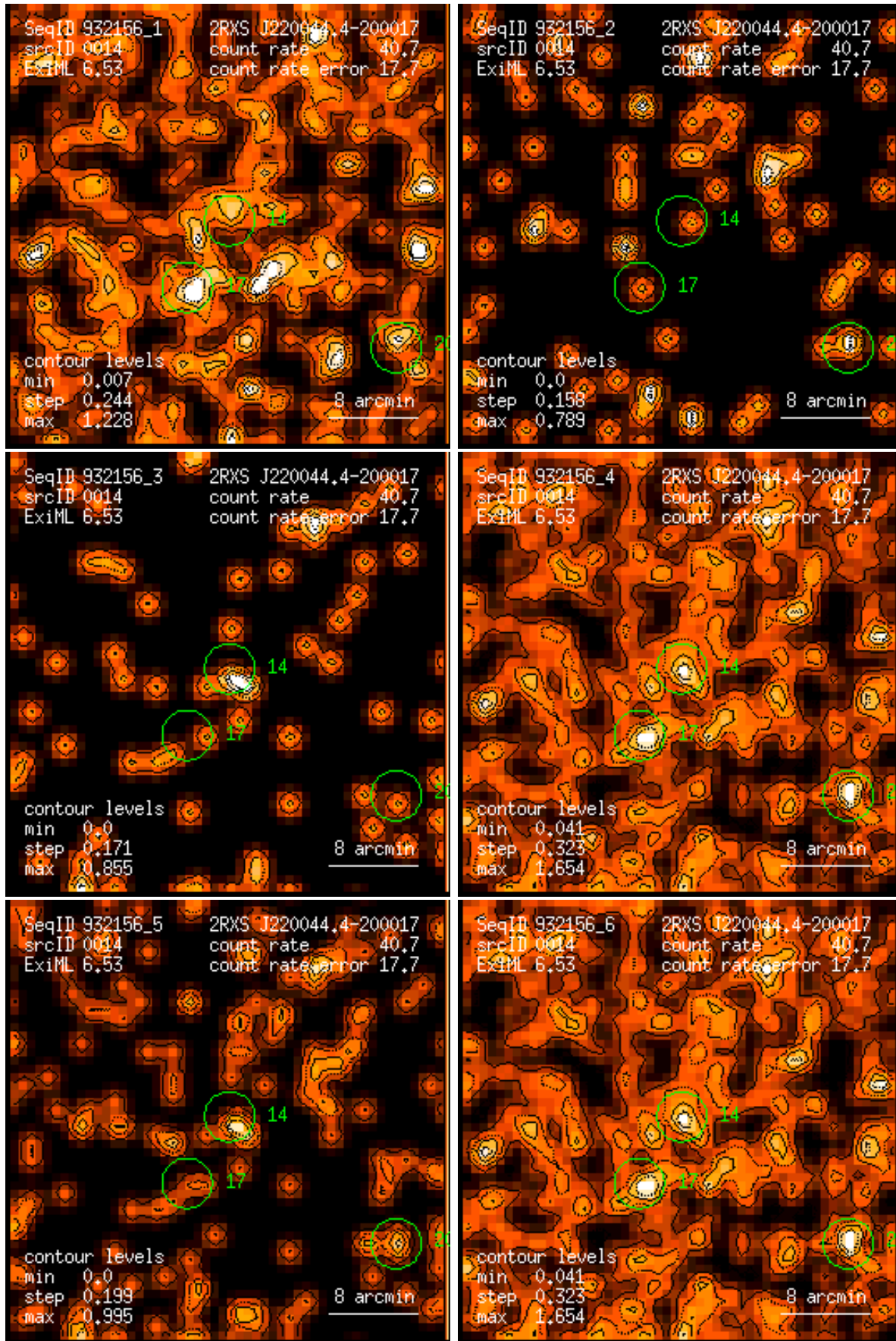
Figure 14: RASS 932156: detection 0014: band rate images, Gaussian filter: (1) PSPC channels 11 – 41, (2) 52 – 90, (3) 91 – 201, (4) 11 – 235, (5) 52 – 201, (6) 11 – 201. Broad band rates in counts/ks. Band rate contour levels in counts/ks/arcmin 2 .
