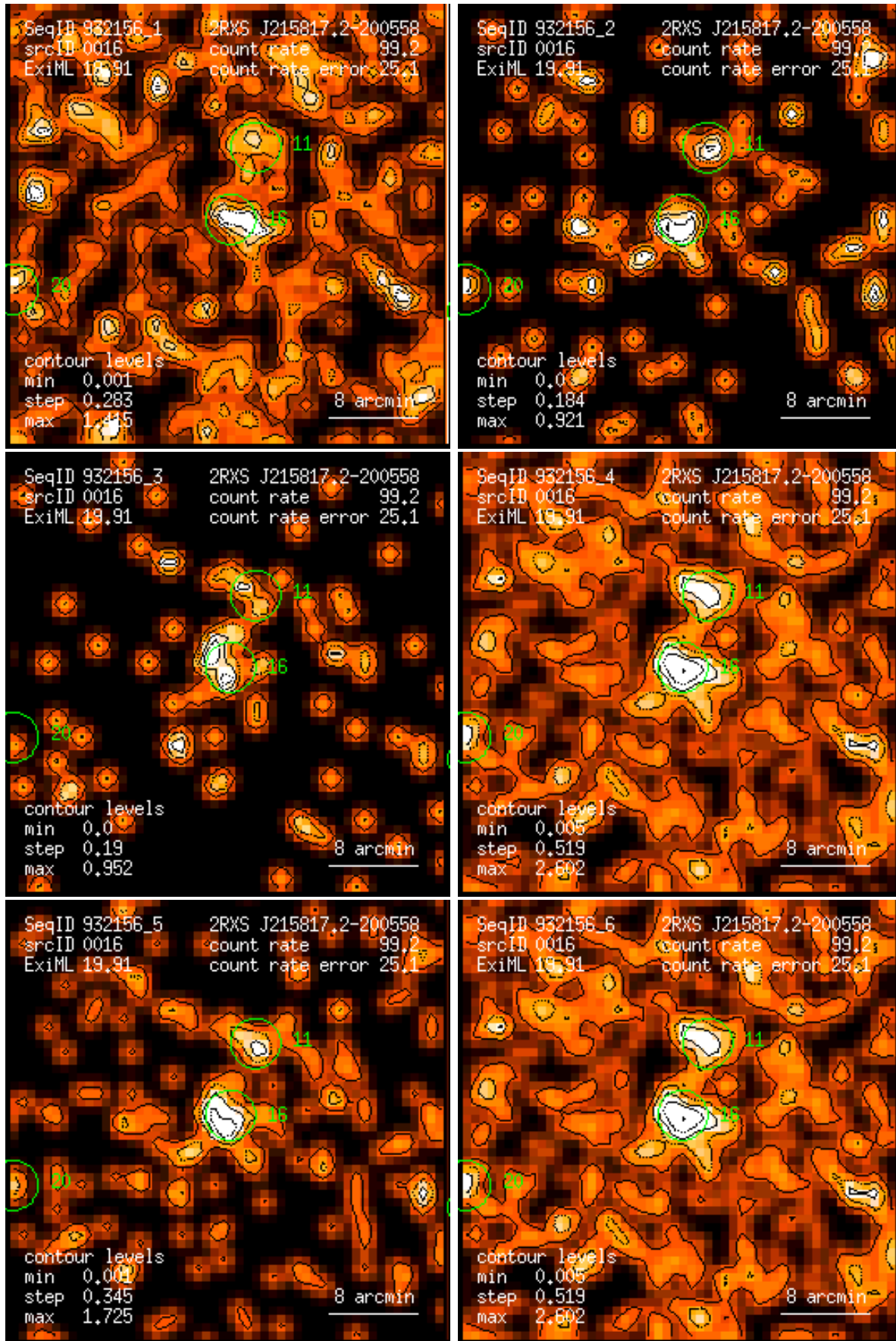
Figure 16: RASS 932156: detection 0016: band rate images, Gaussian filter: (1) PSPC channels 11 – 41, (2) 52 – 90, (3) 91 – 201, (4) 11 – 235, (5) 52 – 201, (6) 11 – 201. Broad band rates in counts/ks. Band rate contour levels in counts/ks/arcmin 2 .
