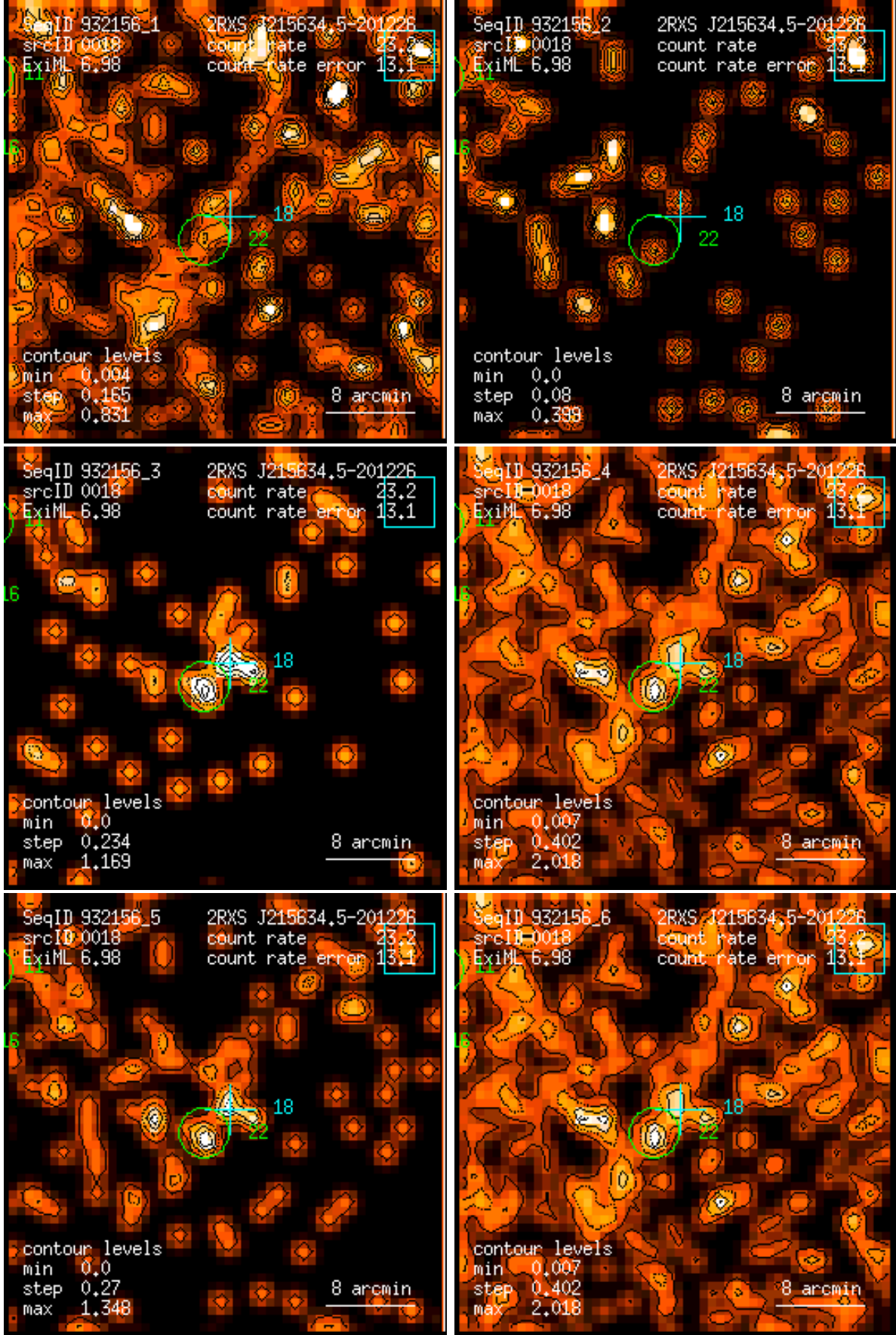
Figure 18: RASS 932156: detection 0018: band rate images, Gaussian filter: (1) PSPC channels 11 – 41, (2) 52 – 90, (3) 91 – 201, (4) 11 – 235, (5) 52 – 201, (6) 11 – 201. Broad band rates in counts/ks. Band rate contour levels in counts/ks/arcmin 2 .
