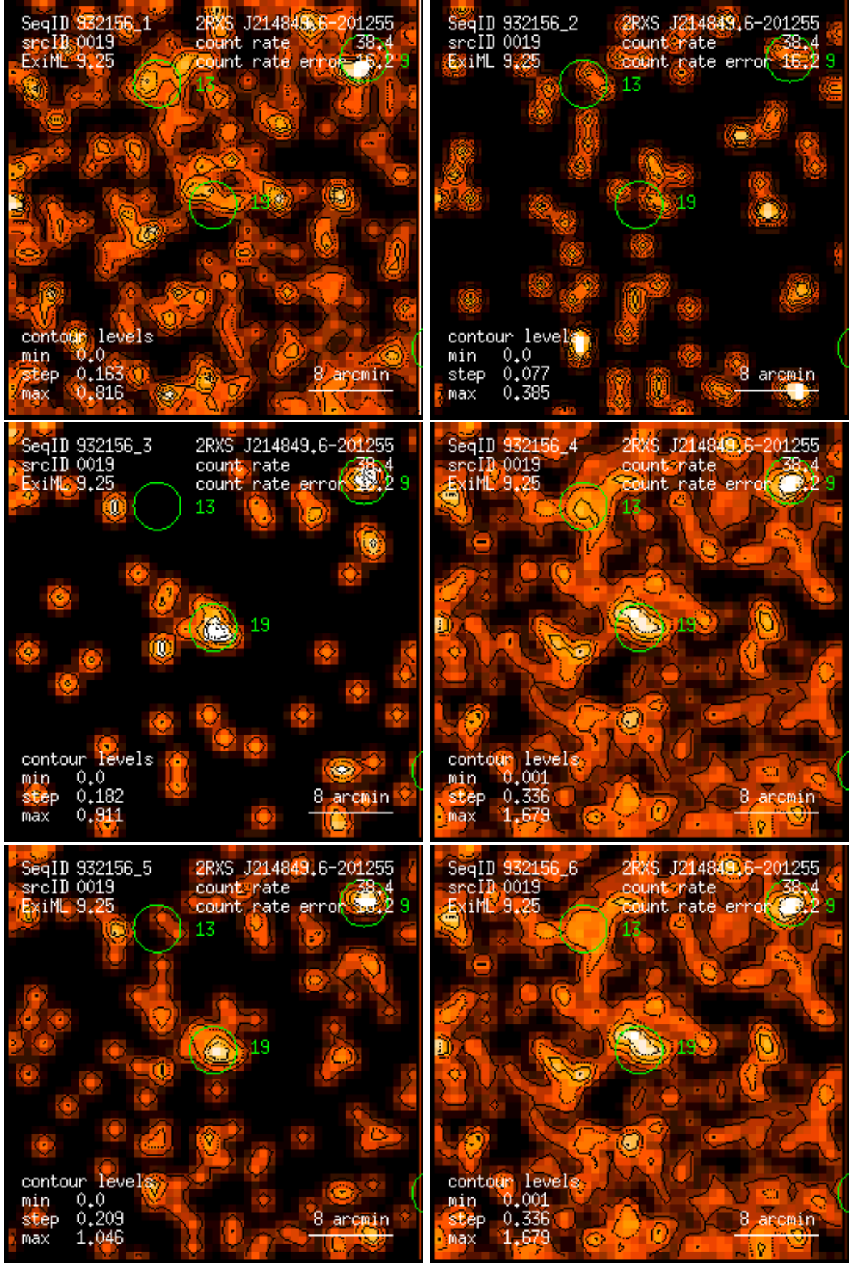
Figure 19: RASS 932156: detection 0019: band rate images, Gaussian filter: (1) PSPC channels 11 – 41, (2) 52 – 90, (3) 91 – 201, (4) 11 – 235, (5) 52 – 201, (6) 11 – 201. Broad band rates in counts/ks. Band rate contour levels in counts/ks/arcmin 2 .
