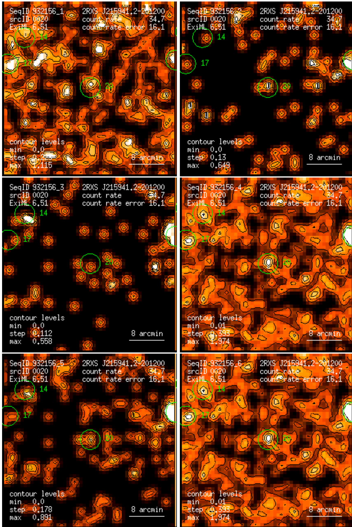
Figure 20: RASS 932156: detection 0020: band rate images, Gaussian filter: (1) PSPC channels 11 – 41, (2) 52 – 90, (3) 91 – 201, (4) 11 – 235, (5) 52 – 201, (6) 11 – 201. Broad band rates in counts/ks. Band rate contour levels in counts/ks/arcmin 2 .
