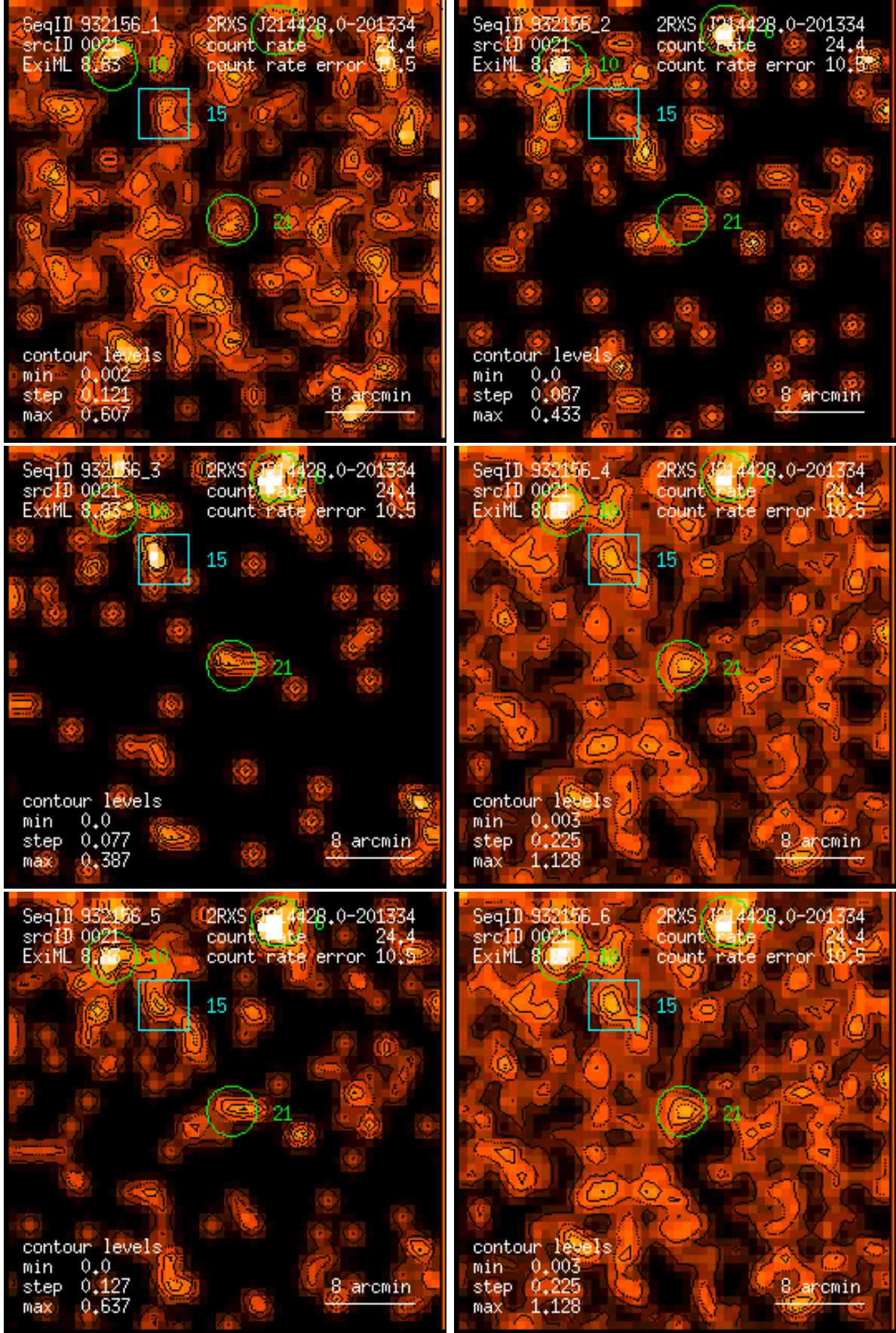
Figure 21: RASS 932156: detection 0021: band rate images, Gaussian filter: (1) PSPC channels 11 – 41, (2) 52 – 90, (3) 91 – 201, (4) 11 – 235, (5) 52 – 201, (6) 11 – 201. Broad band rates in counts/ks. Band rate contour levels in counts/ks/arcmin 2 .
