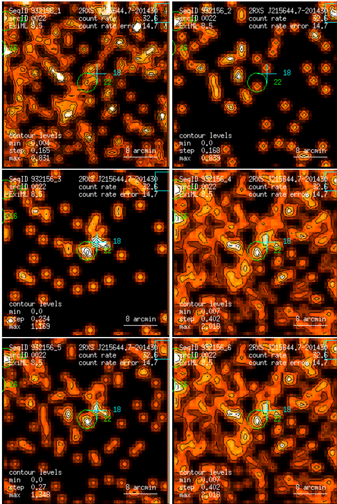
Figure 22: RASS 932156: detection 0022: band rate images, Gaussian filter: (1) PSPC channels 11 – 41, (2) 52 – 90, (3) 91 – 201, (4) 11 – 235, (5) 52 – 201, (6) 11 – 201. Broad band rates in counts/ks. Band rate contour levels in counts/ks/arcmin 2 .
