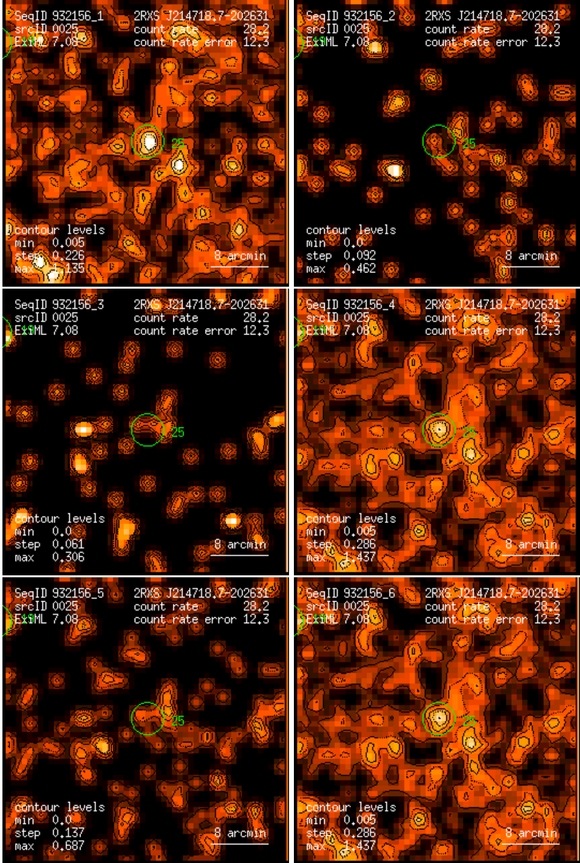
Figure 25: RASS 932156: detection 0025: band rate images, Gaussian filter: (1) PSPC channels 11 – 41, (2) 52 – 90, (3) 91 – 201, (4) 11 – 235, (5) 52 – 201, (6) 11 – 201. Broad band rates in counts/ks. Band rate contour levels in counts/ks/arcmin 2 .
