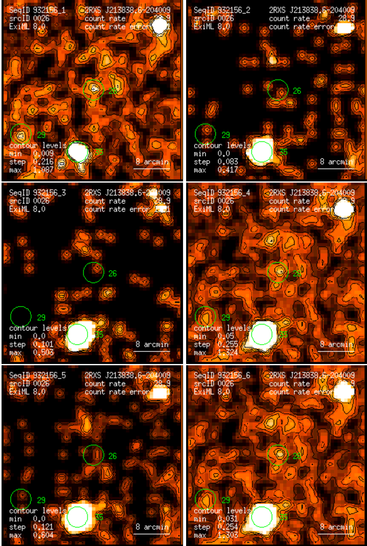
Figure 26: RASS 932156: detection 0026: band rate images, Gaussian filter: (1) PSPC channels 11 – 41, (2) 52 – 90, (3) 91 – 201, (4) 11 – 235, (5) 52 – 201, (6) 11 – 201. Broad band rates in counts/ks. Band rate contour levels in counts/ks/arcmin 2 .
