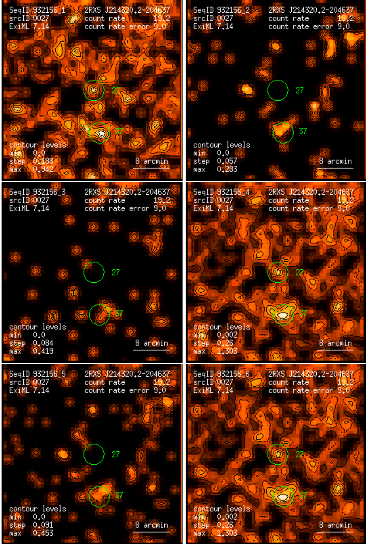
Figure 27: RASS 932156: detection 0027: band rate images, Gaussian filter: (1) PSPC channels 11 – 41, (2) 52 – 90, (3) 91 – 201, (4) 11 – 235, (5) 52 – 201, (6) 11 – 201. Broad band rates in counts/ks. Band rate contour levels in counts/ks/arcmin 2 .
