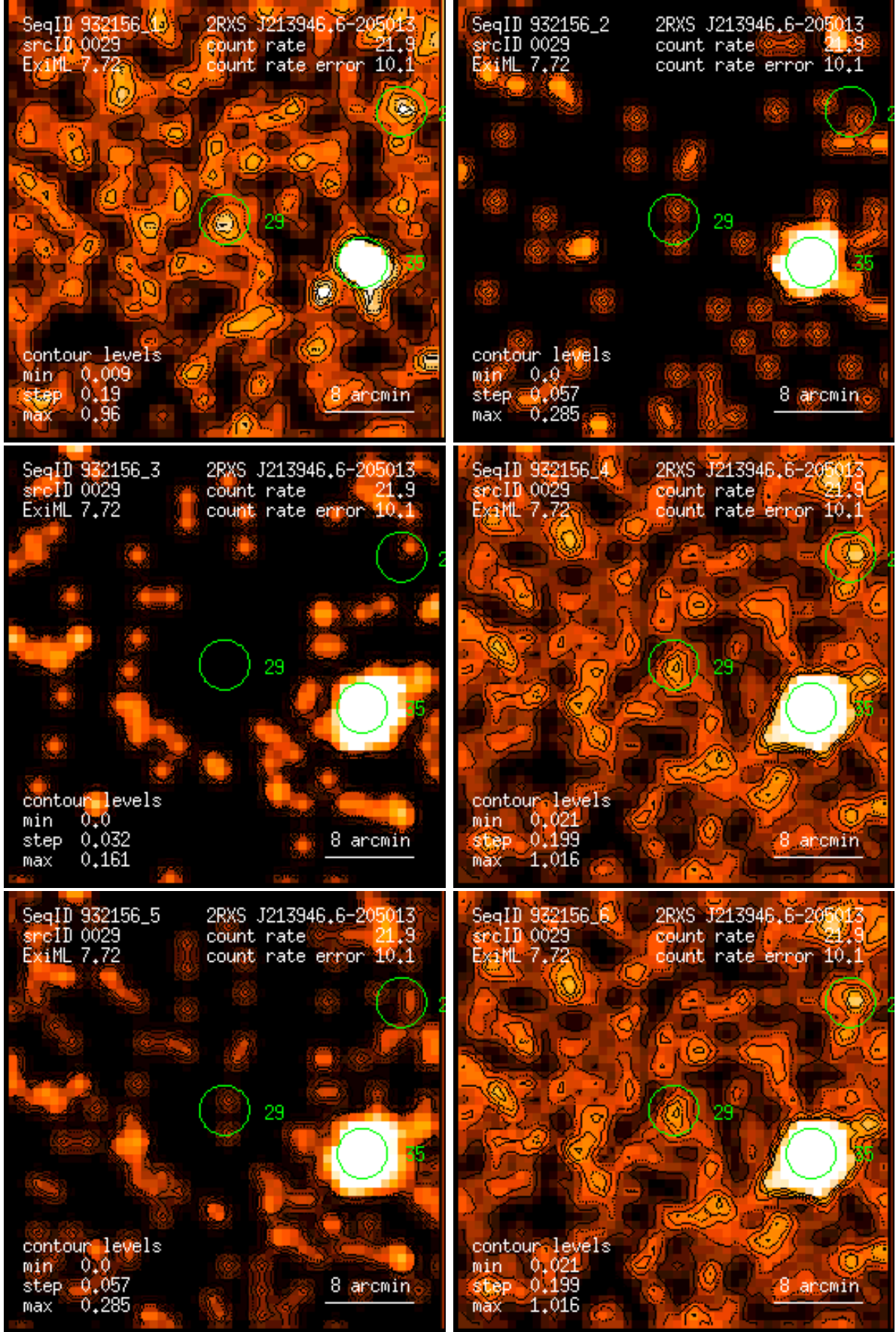
Figure 29: RASS 932156: detection 0029: band rate images, Gaussian filter: (1) PSPC channels 11 – 41, (2) 52 – 90, (3) 91 – 201, (4) 11 – 235, (5) 52 – 201, (6) 11 – 201. Broad band rates in counts/ks. Band rate contour levels in counts/ks/arcmin 2 .
