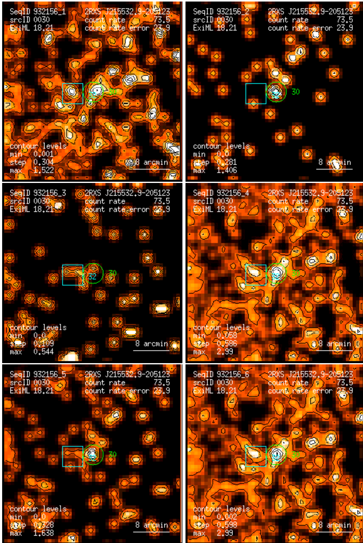
Figure 30: RASS 932156: detection 0030: band rate images, Gaussian filter: (1) PSPC channels 11 – 41, (2) 52 – 90, (3) 91 – 201, (4) 11 – 235, (5) 52 – 201, (6) 11 – 201. Broad band rates in counts/ks. Band rate contour levels in counts/ks/arcmin 2 .
