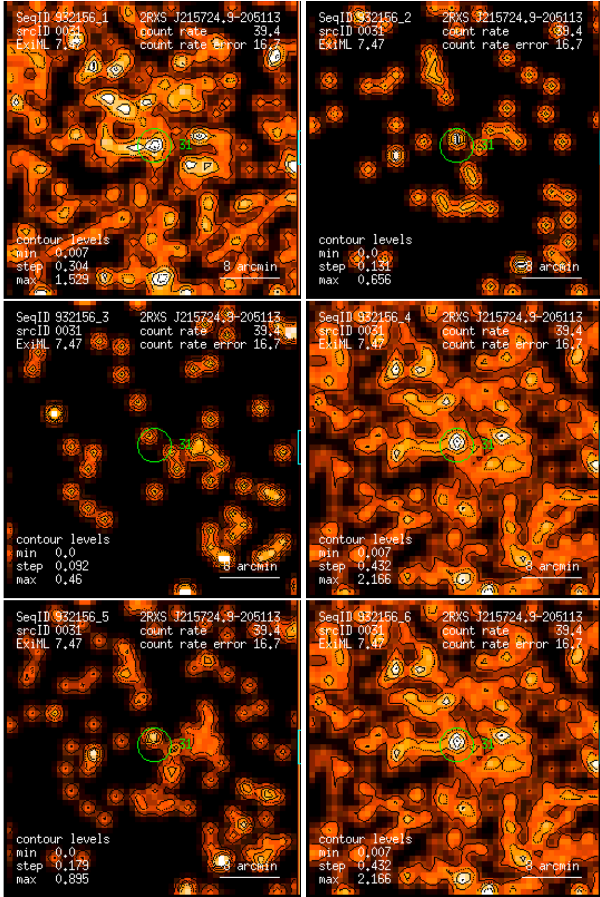
Figure 31: RASS 932156: detection 0031: band rate images, Gaussian filter: (1) PSPC channels 11 – 41, (2) 52 – 90, (3) 91 – 201, (4) 11 – 235, (5) 52 – 201, (6) 11 – 201. Broad band rates in counts/ks. Band rate contour levels in counts/ks/arcmin 2 .
