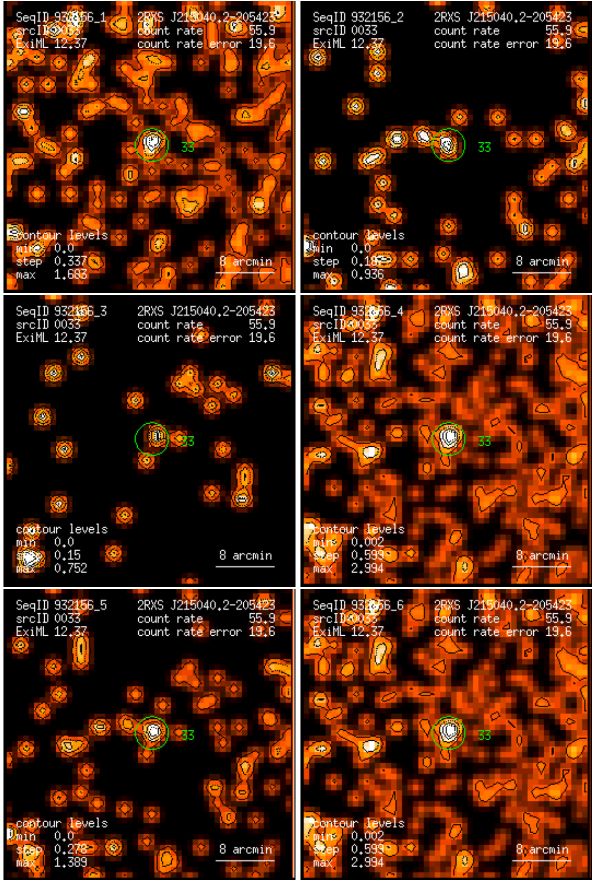
Figure 33: RASS 932156: detection 0033: band rate images, Gaussian filter: (1) PSPC channels 11 – 41, (2) 52 – 90, (3) 91 – 201, (4) 11 – 235, (5) 52 – 201, (6) 11 – 201. Broad band rates in counts/ks. Band rate contour levels in counts/ks/arcmin 2 .
