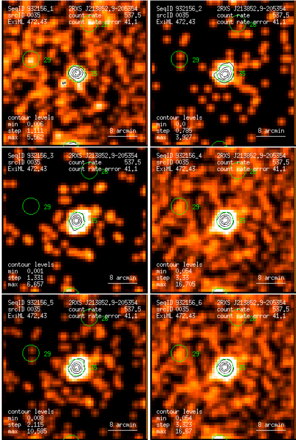
Figure 35: RASS 932156: detection 0035: band rate images, Gaussian filter: (1) PSPC channels 11 – 41, (2) 52 – 90, (3) 91 – 201, (4) 11 – 235, (5) 52 – 201, (6) 11 – 201. Broad band rates in counts/ks. Band rate contour levels in counts/ks/arcmin 2 .
