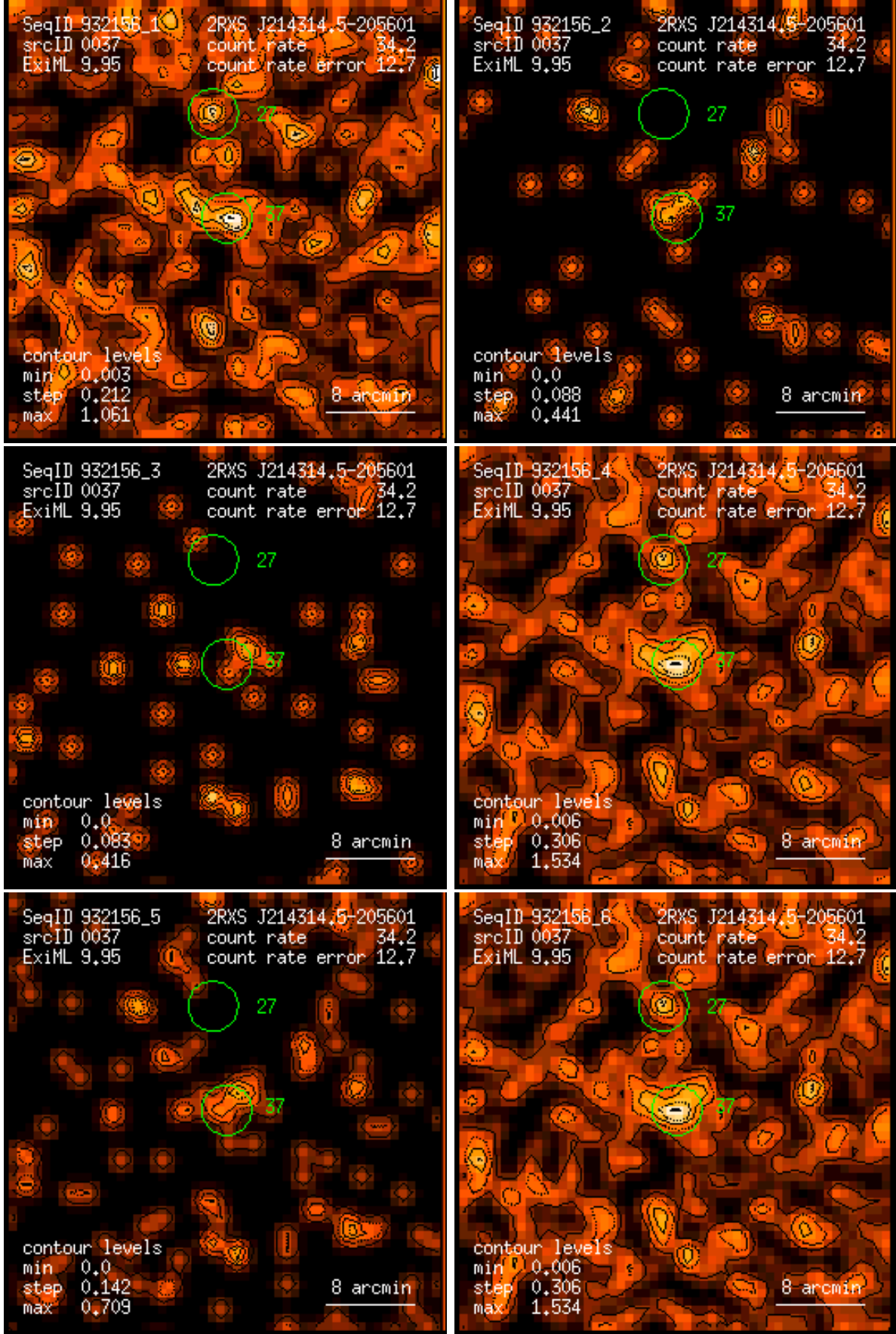
Figure 37: RASS 932156: detection 0037: band rate images, Gaussian filter: (1) PSPC channels 11 – 41, (2) 52 – 90, (3) 91 – 201, (4) 11 – 235, (5) 52 – 201, (6) 11 – 201. Broad band rates in counts/ks. Band rate contour levels in counts/ks/arcmin 2 .
