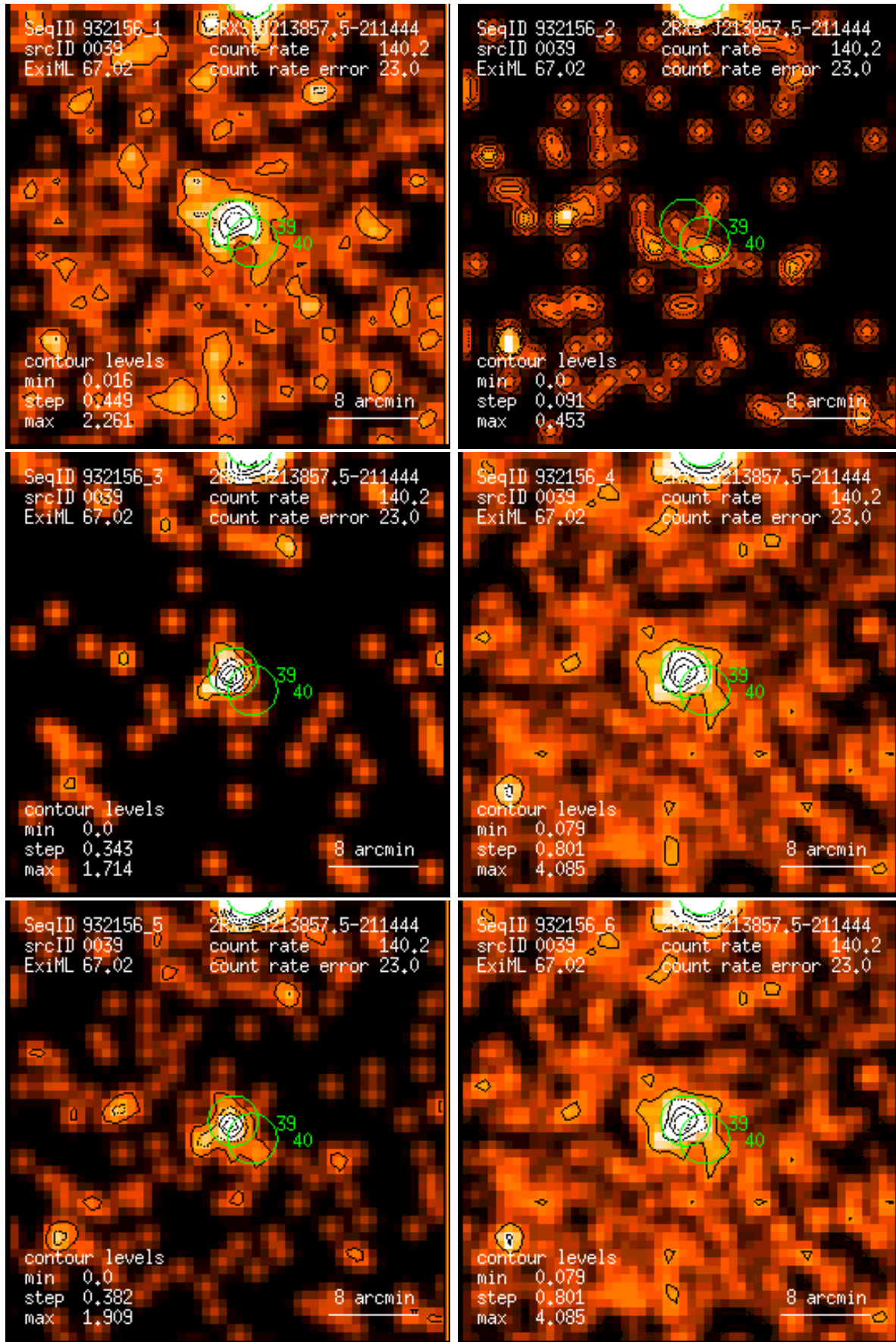
Figure 39: RASS 932156: detection 0039: band rate images, Gaussian filter: (1) PSPC channels 11 – 41, (2) 52 – 90, (3) 91 – 201, (4) 11 – 235, (5) 52 – 201, (6) 11 – 201. Broad band rates in counts/ks. Band rate contour levels in counts/ks/arcmin 2 .
