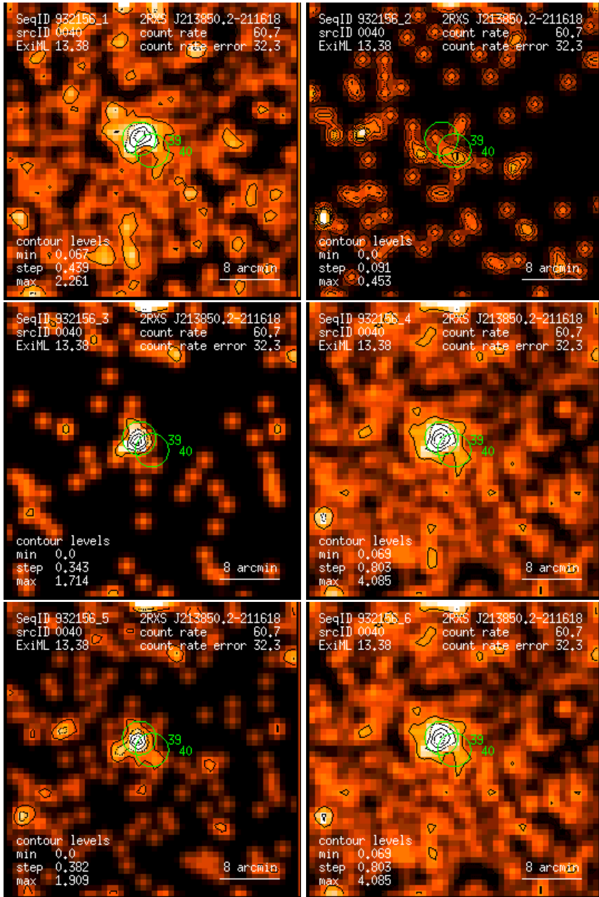
Figure 40: RASS 932156: detection 0040: band rate images, Gaussian filter: (1) PSPC channels 11 – 41, (2) 52 – 90, (3) 91 – 201, (4) 11 – 235, (5) 52 – 201, (6) 11 – 201. Broad band rates in counts/ks. Band rate contour levels in counts/ks/arcmin 2 .
