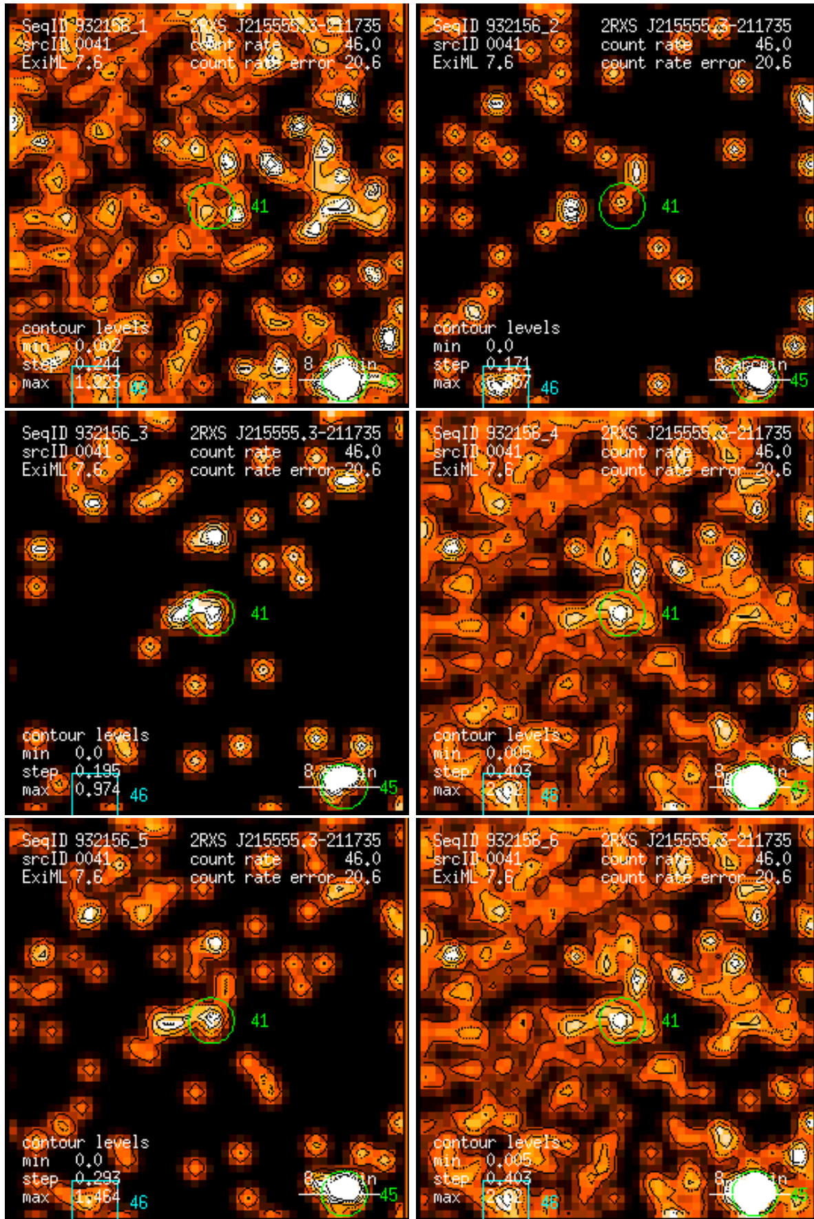
Figure 41: RASS 932156: detection 0041: band rate images, Gaussian filter: (1) PSPC channels 11 – 41, (2) 52 – 90, (3) 91 – 201, (4) 11 – 235, (5) 52 – 201, (6) 11 – 201. Broad band rates in counts/ks. Band rate contour levels in counts/ks/arcmin 2 .
