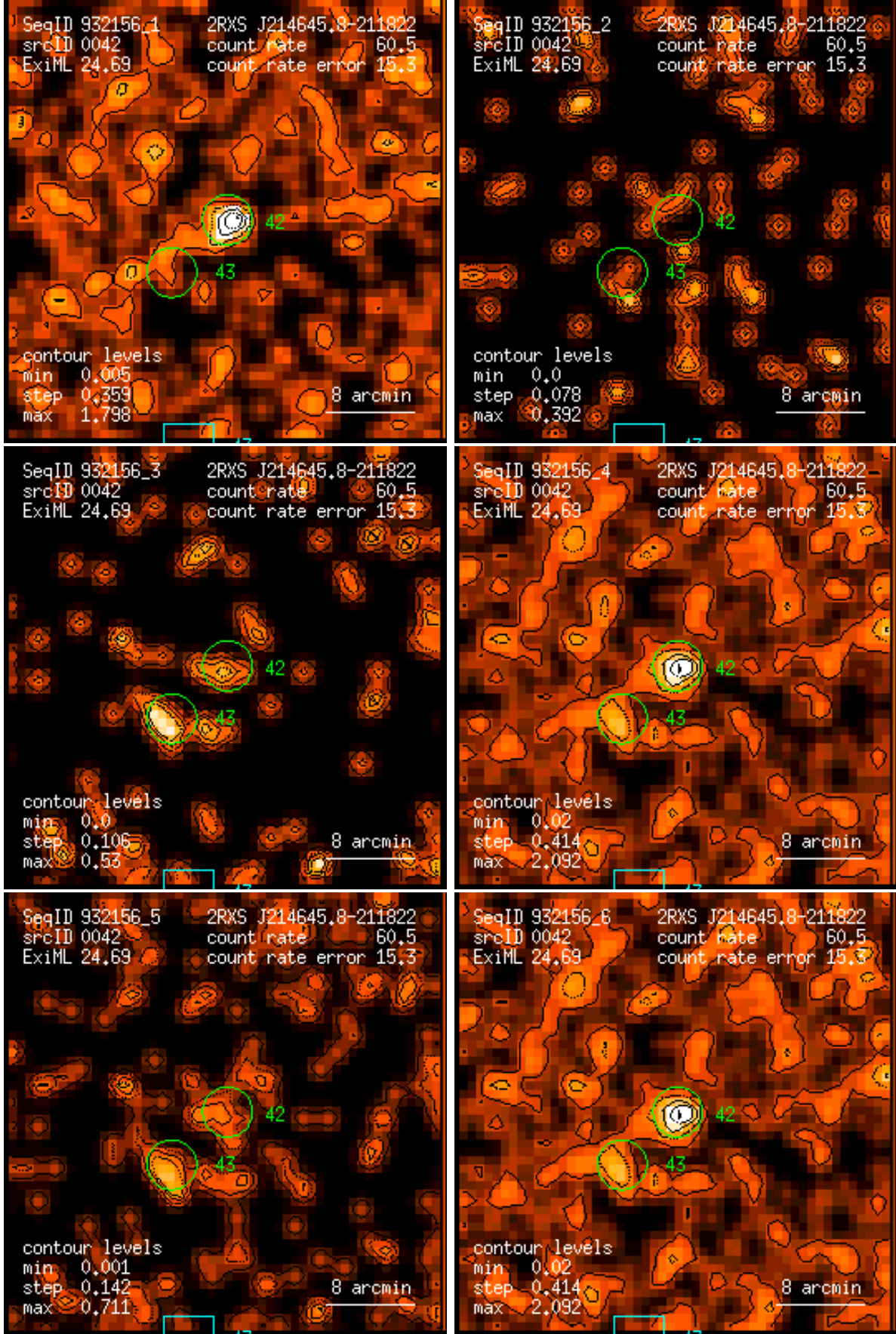
Figure 42: RASS 932156: detection 0042: band rate images, Gaussian filter: (1) PSPC channels 11 – 41, (2) 52 – 90, (3) 91 – 201, (4) 11 – 235, (5) 52 – 201, (6) 11 – 201. Broad band rates in counts/ks. Band rate contour levels in counts/ks/arcmin 2 .
