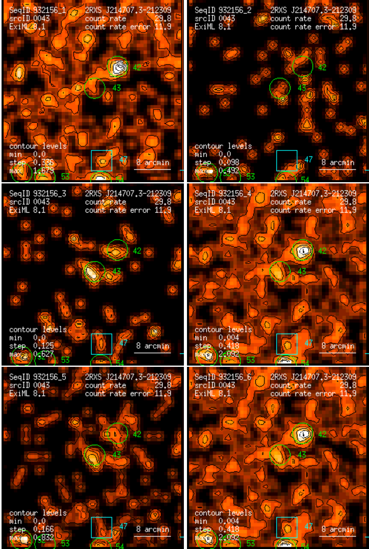
Figure 43: RASS 932156: detection 0043: band rate images, Gaussian filter: (1) PSPC channels 11 – 41, (2) 52 – 90, (3) 91 – 201, (4) 11 – 235, (5) 52 – 201, (6) 11 – 201. Broad band rates in counts/ks. Band rate contour levels in counts/ks/arcmin 2 .
