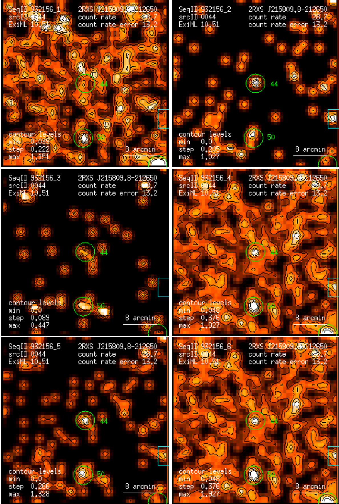
Figure 44: RASS 932156: detection 0044: band rate images, Gaussian filter: (1) PSPC channels 11 – 41, (2) 52 – 90, (3) 91 – 201, (4) 11 – 235, (5) 52 – 201, (6) 11 – 201. Broad band rates in counts/ks. Band rate contour levels in counts/ks/arcmin 2 .
