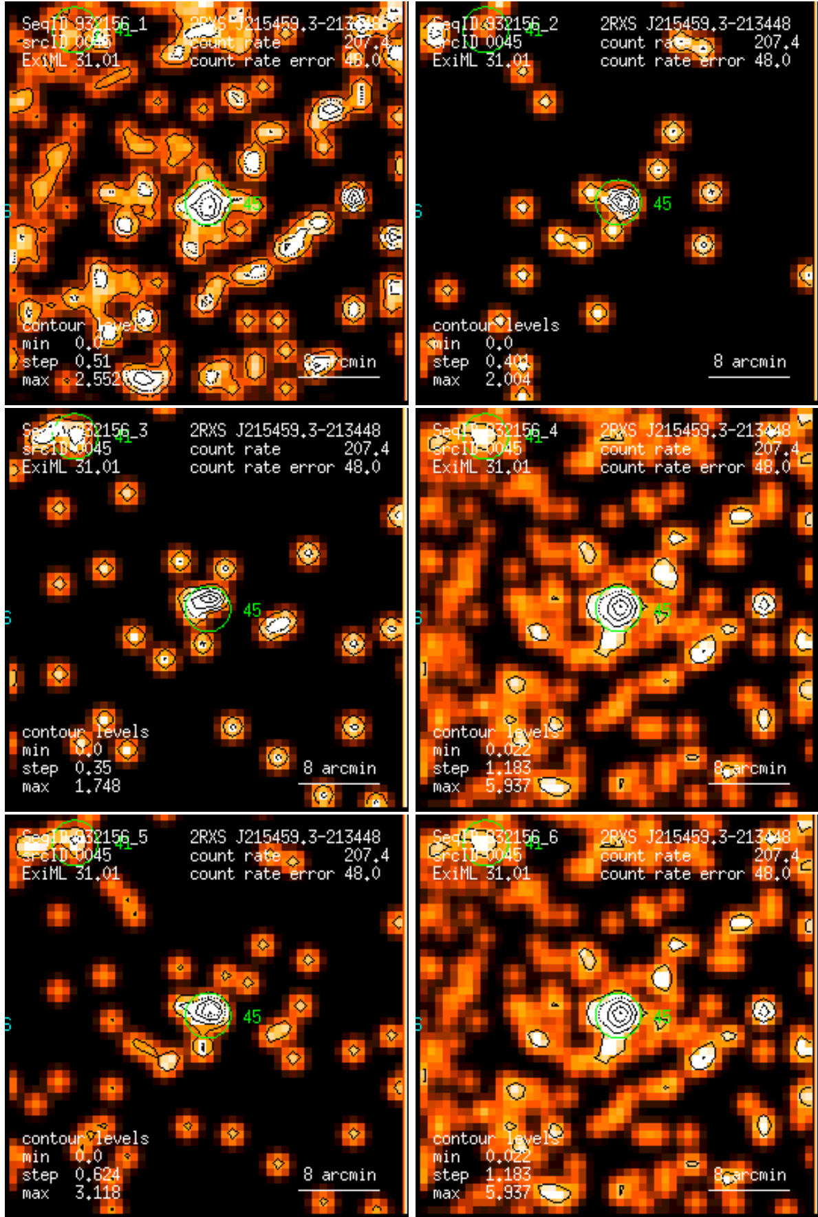
Figure 45: RASS 932156: detection 0045: band rate images, Gaussian filter: (1) PSPC channels 11 – 41, (2) 52 – 90, (3) 91 – 201, (4) 11 – 235, (5) 52 – 201, (6) 11 – 201. Broad band rates in counts/ks. Band rate contour levels in counts/ks/arcmin 2 .
